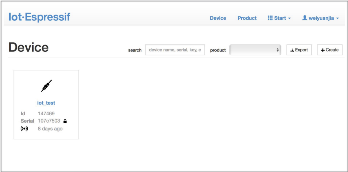
图 23: 点击 “Device”
