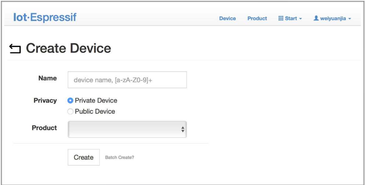
图 24: 点击 “Create”
