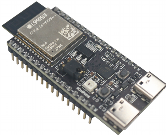
ESP32-C6-DevKitC-1
