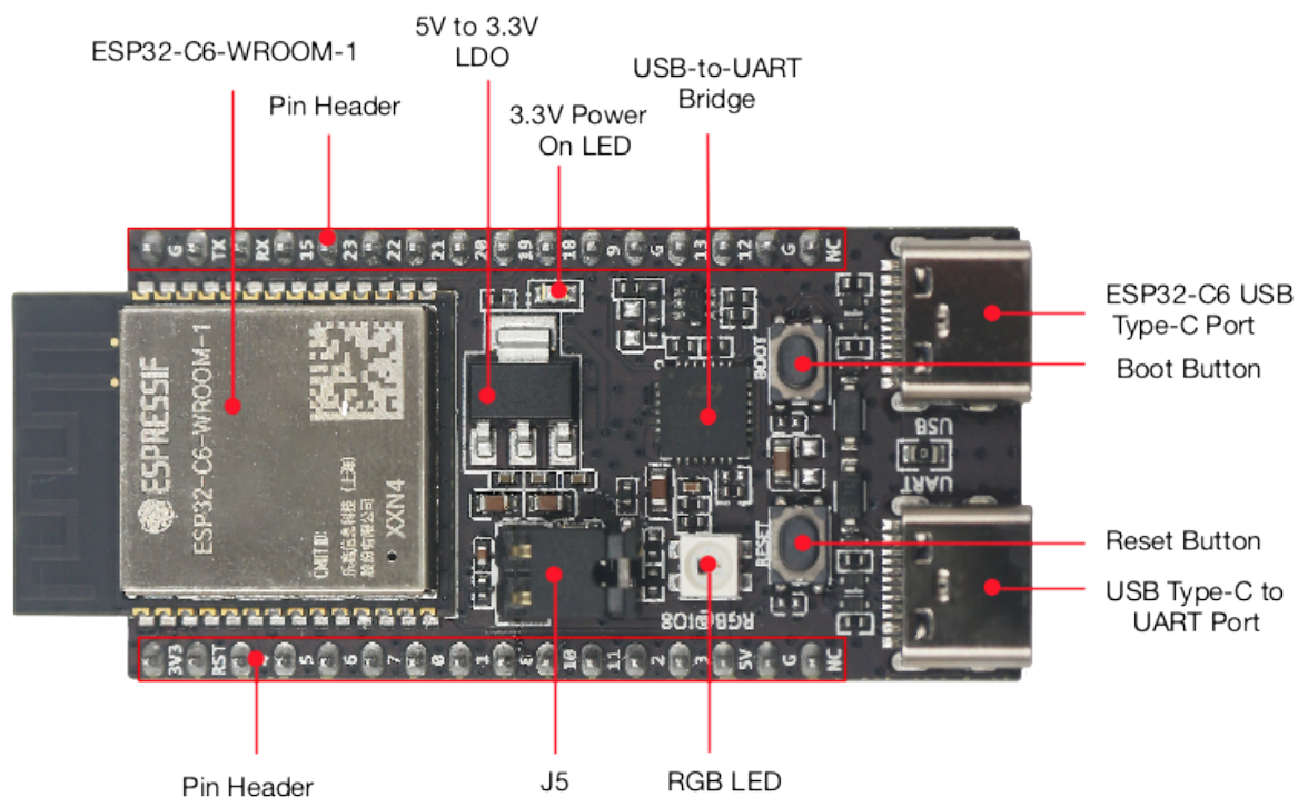
Fig. 2: ESP32-C6-DevKitC-1 - front
