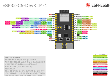
Fig. 4: ESP32-C6-DevKitM-1 Pin Layout (click to enlarge)
