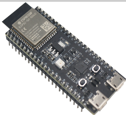
ESP32-S2-DevKitC-1
