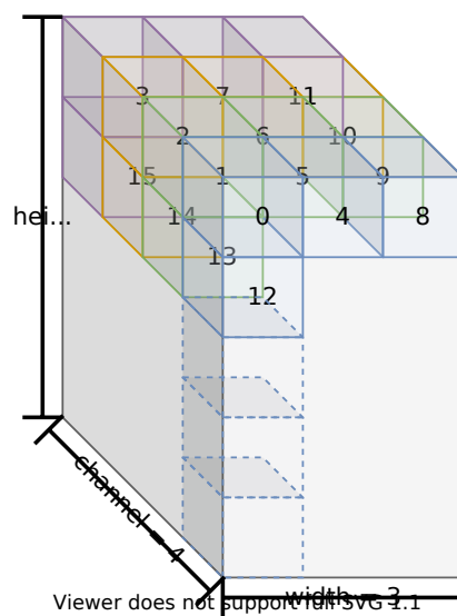
Fig. 1: 3D Tensor
