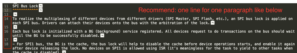
Fig. 10: One line per paragraph - recommended (click to enlarge)
