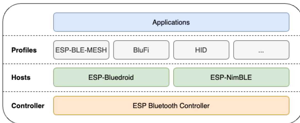
Fig. 2: ESP32-C5 Bluetooth LE Stack Architecture
