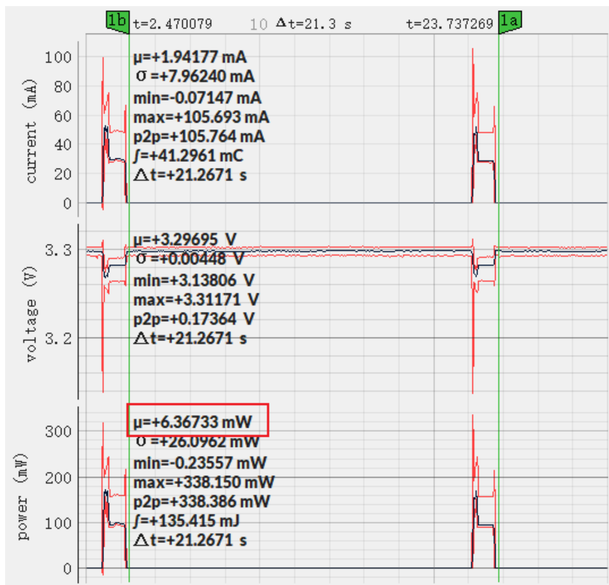
Fig. 41: Power Consumption of ESP32-S3-WROOM-1 (click to enlarge)
