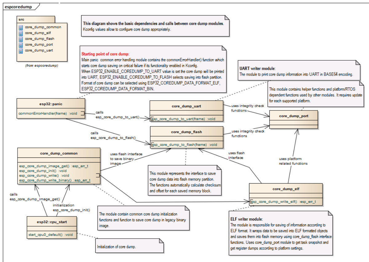
Fig. 38: Core Dump Implementation Overview
