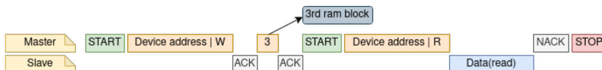
Fig. 13: Get data from I2C slave RAM
