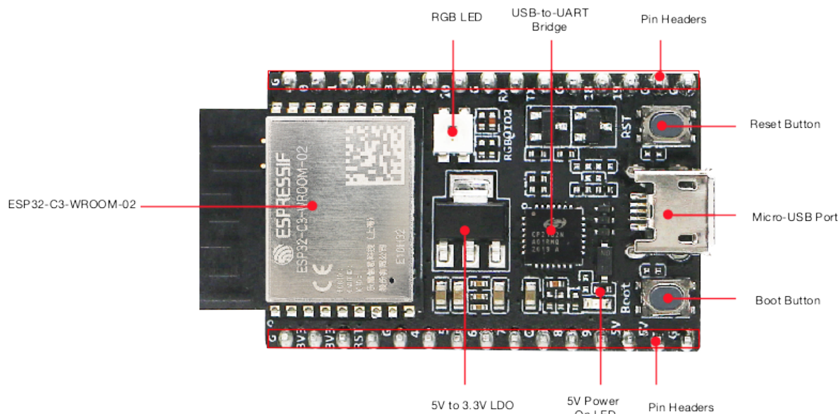
Fig. 7: ESP32-C3-DevKitC-02 - front
