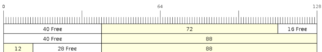
Fig. 33: Wrap around in byte buffers
