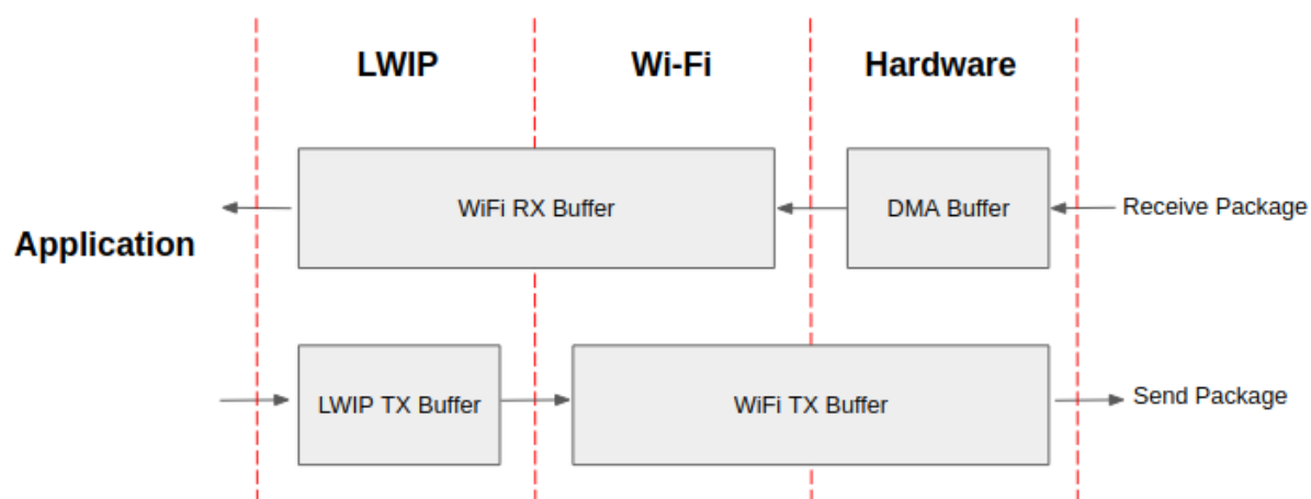
Fig. 62: ESP32 datapath
