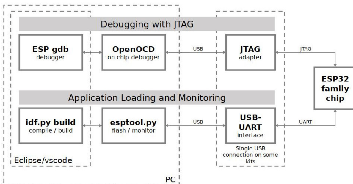
Fig. 58: JTAG debugging - overview diagram
