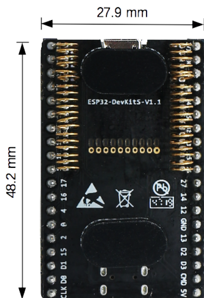
Fig. 4: ESP32-DevKitS-R board dimensions - back
