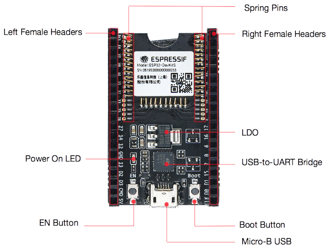
Fig. 1: ESP32-DevKitS - front
