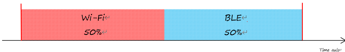
Fig. 68: Time Slice Under the Status of Wi-Fi CONNECTED and BLE CONNECTED
