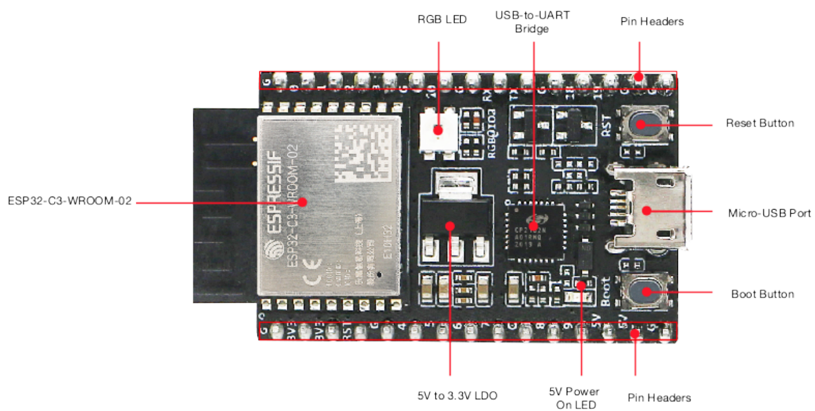
Fig. 6: ESP32-C3-DevKitC-02 - front
