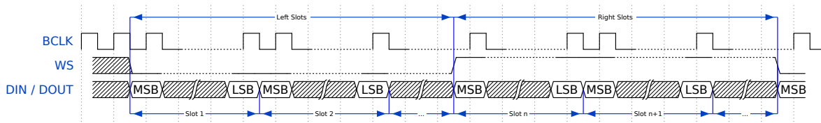
TDM MSB Timing Diagram
