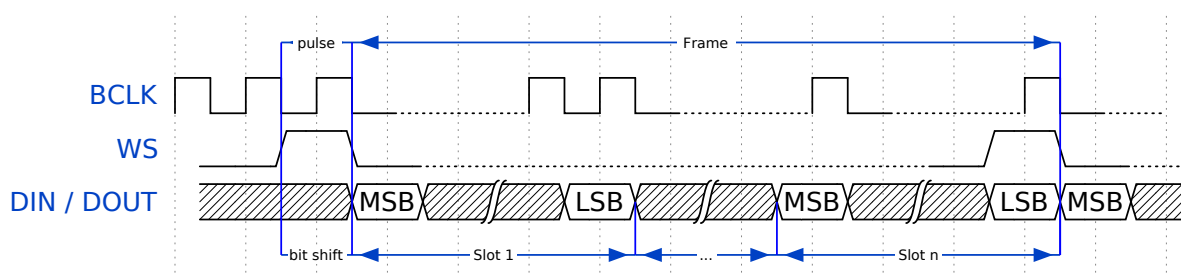
TDM PCM (short) Timing Diagram
