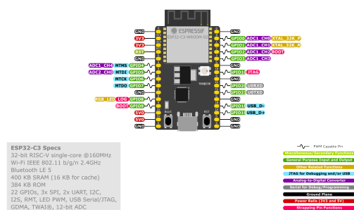
Fig. 8: ESP32-C3-DevKitC-02 Pin Layout (click to enlarge)
