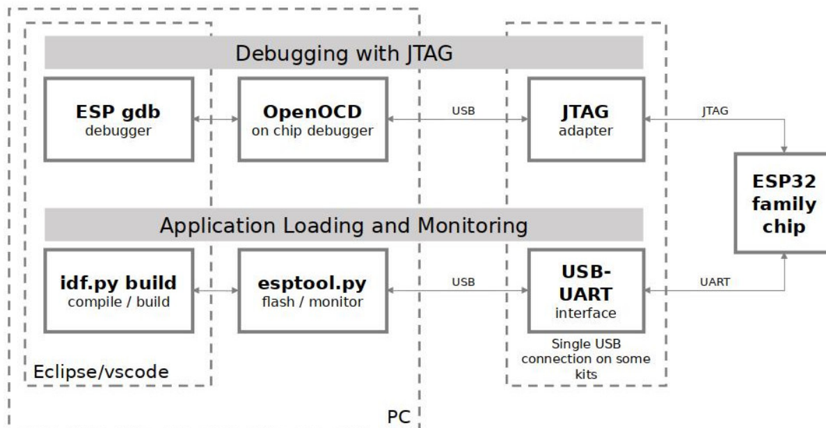
Fig. 37: JTAG debugging - overview diagram
