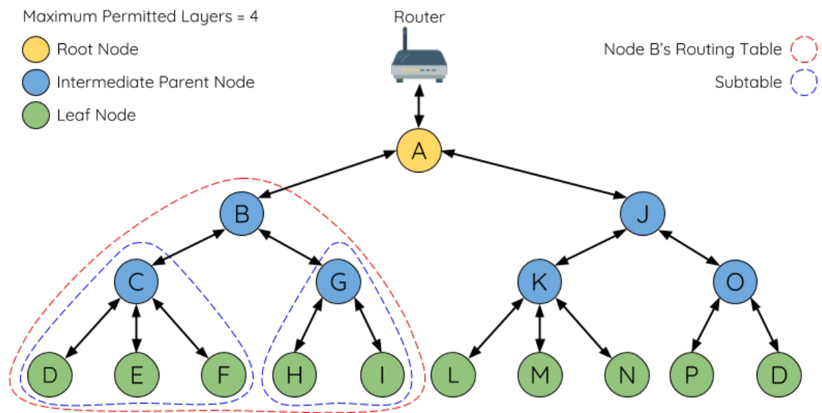
Fig. 46: ESP-WIFI-MESH Routing Tables Example
