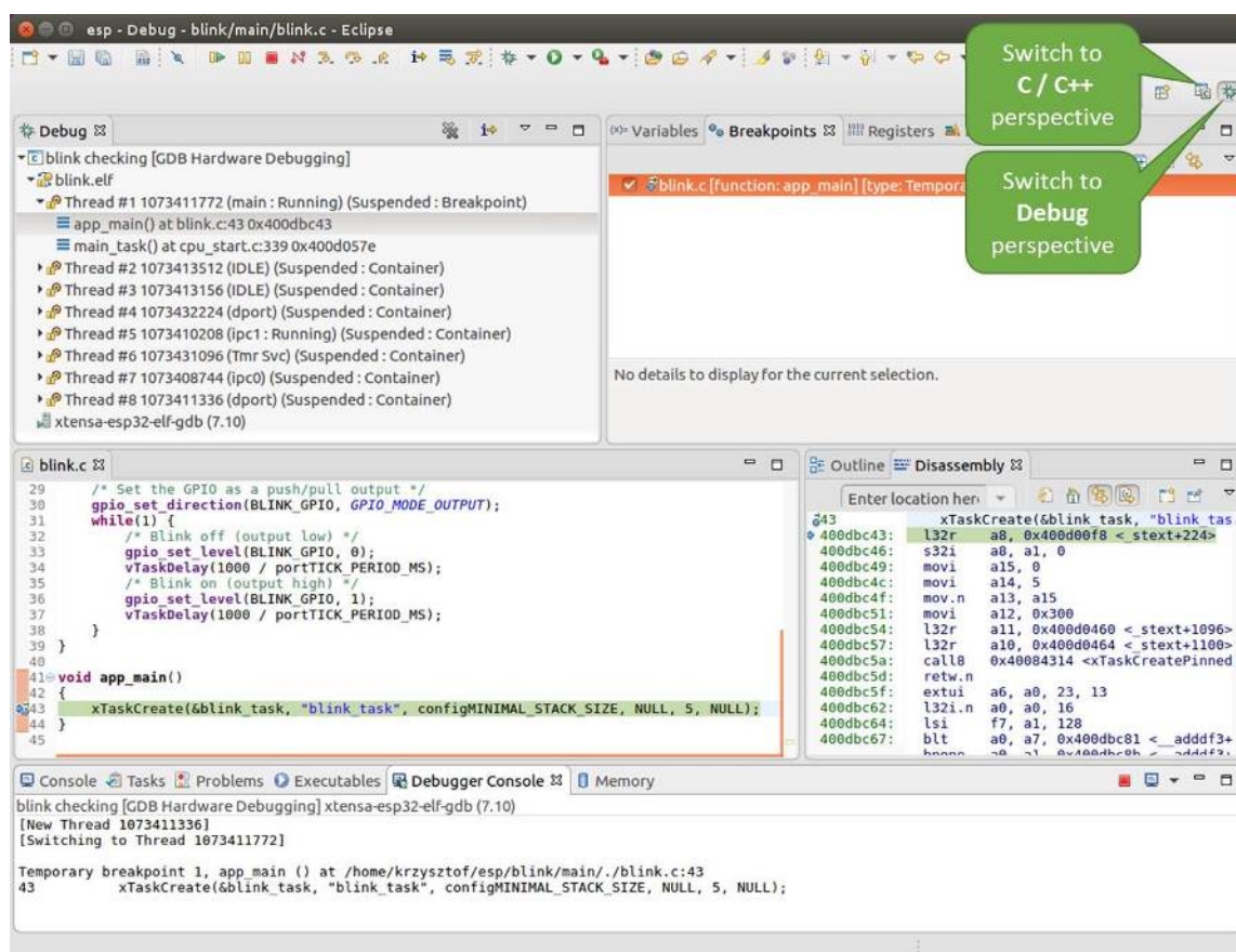
Fig. 62: Debug Perspective in Eclipse
