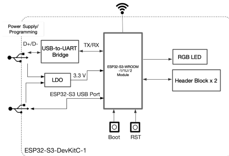
Fig. 3: ESP32-S3-DevKitC-1 (click to enlarge)
