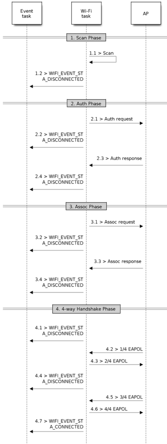
Fig. 81: Wi-Fi Station Connecting Process
