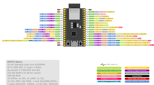
Fig. 53: ESP32-DevKitM-1 (click to enlarge)
