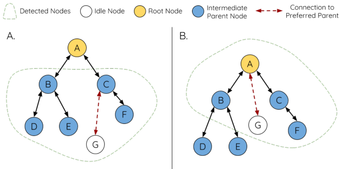
Fig. 28: Preferred Parent Node Selection
