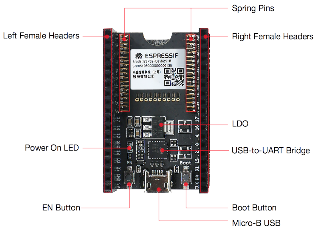
Fig. 2: ESP32-DevKitS-R - front
