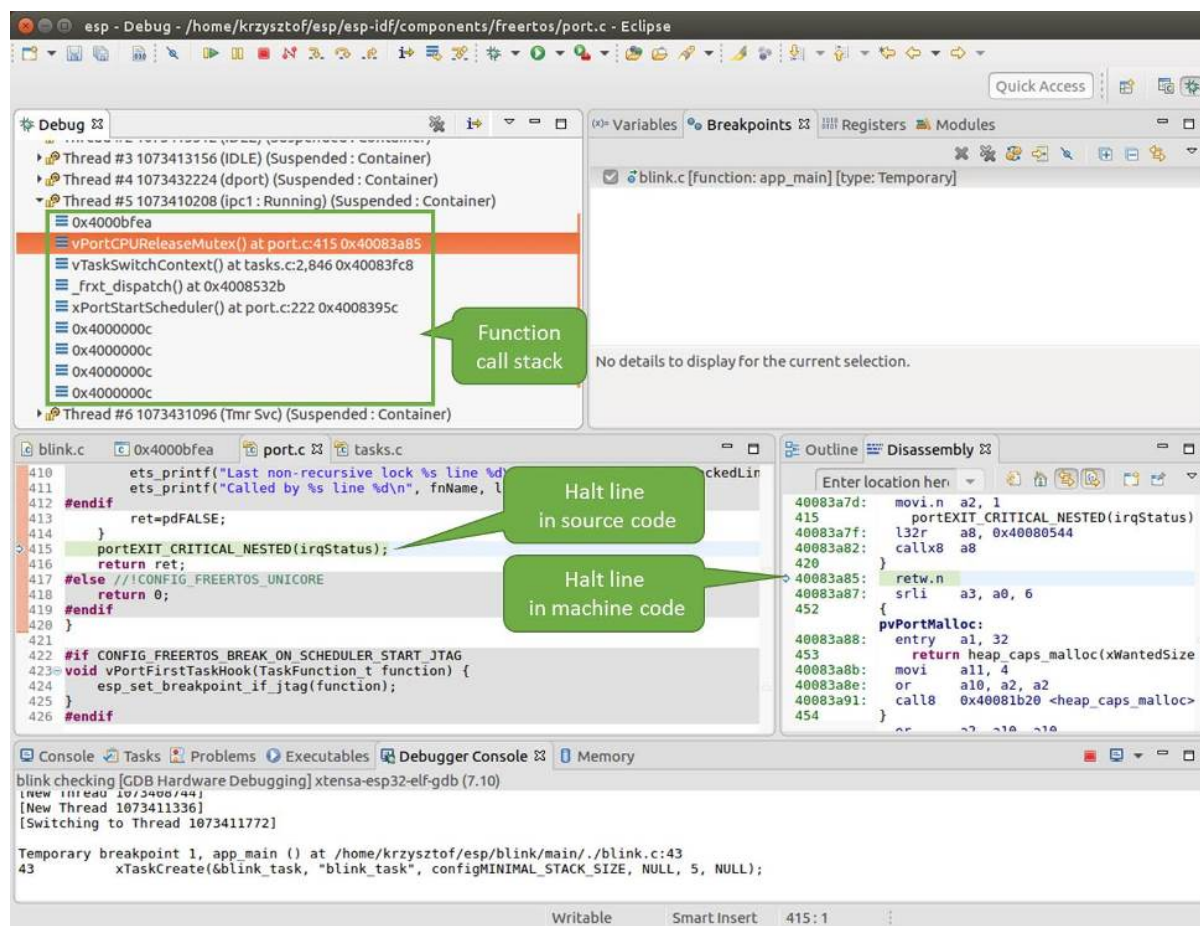
Fig. 68: Navigate through the call stack
