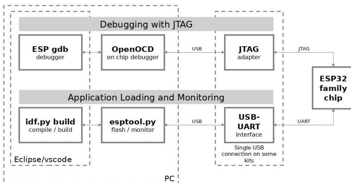
Fig. 60: JTAG debugging - overview diagram
