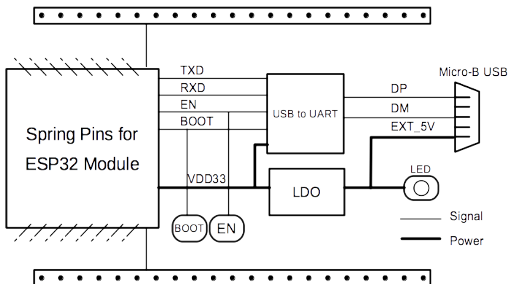
Fig. 5: ESP32-DevKitS(-R) (click to enlarge)
