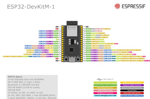
Fig. 8: ESP32-DevKitM-1 (click to enlarge)
