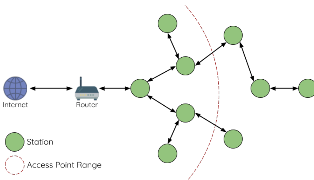
Fig. 44: ESP-WIFI-MESH Network Architecture
