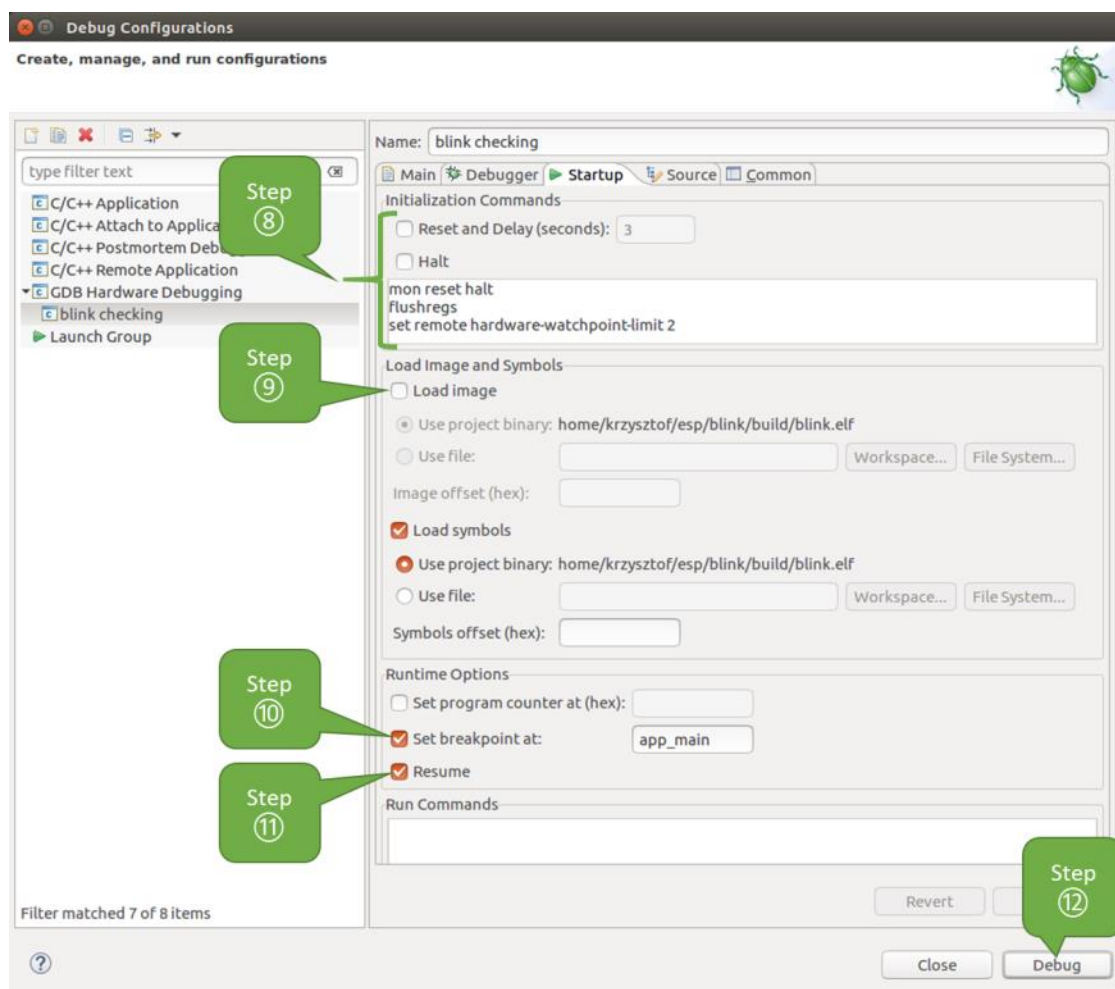
Fig. 64: Configuration of GDB Hardware Debugging - Startup tab
