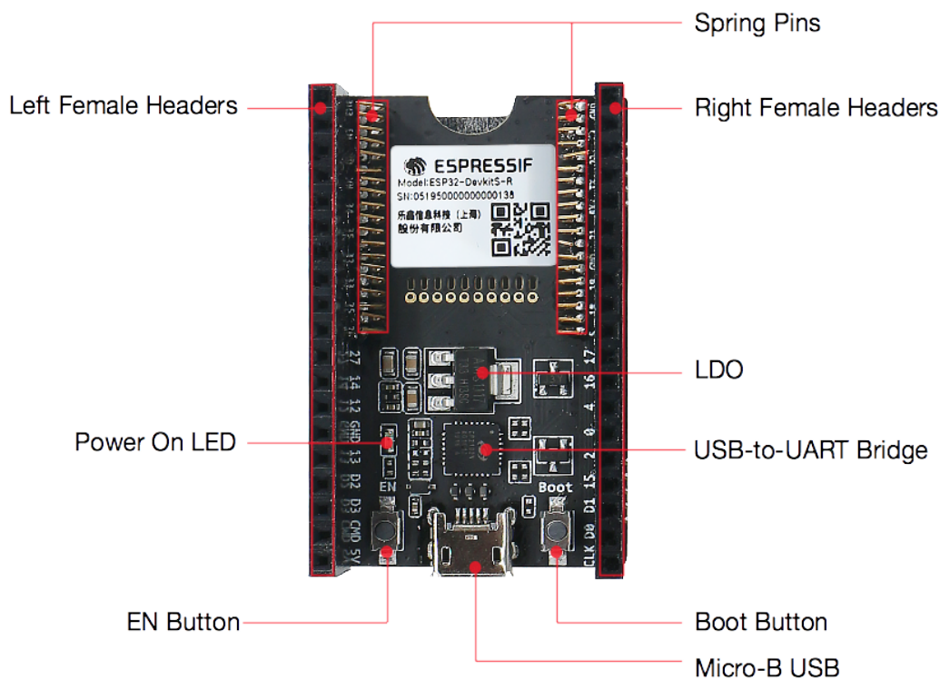
Fig. 2: ESP32-DevKitS-R - front
