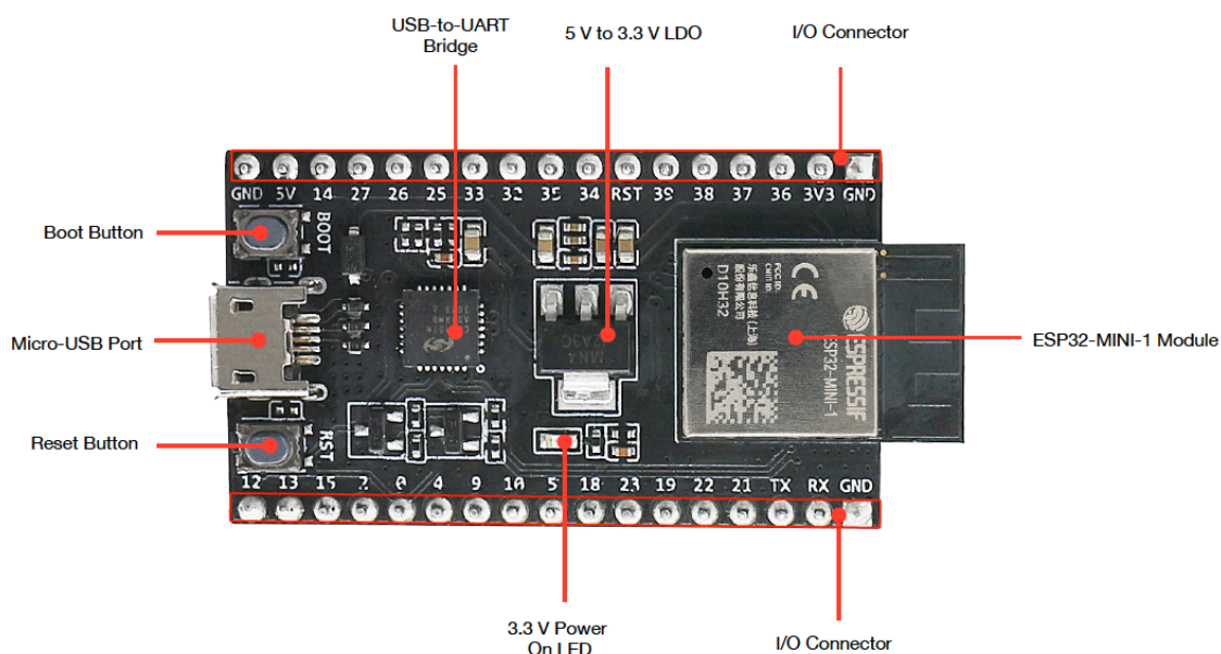
Fig. 6: ESP32-DevKitM-1 - front
