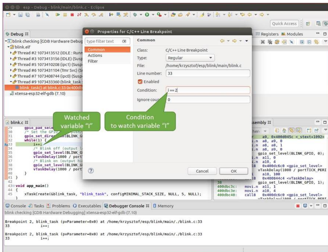
Fig. 27: Setting a conditional breakpoint
