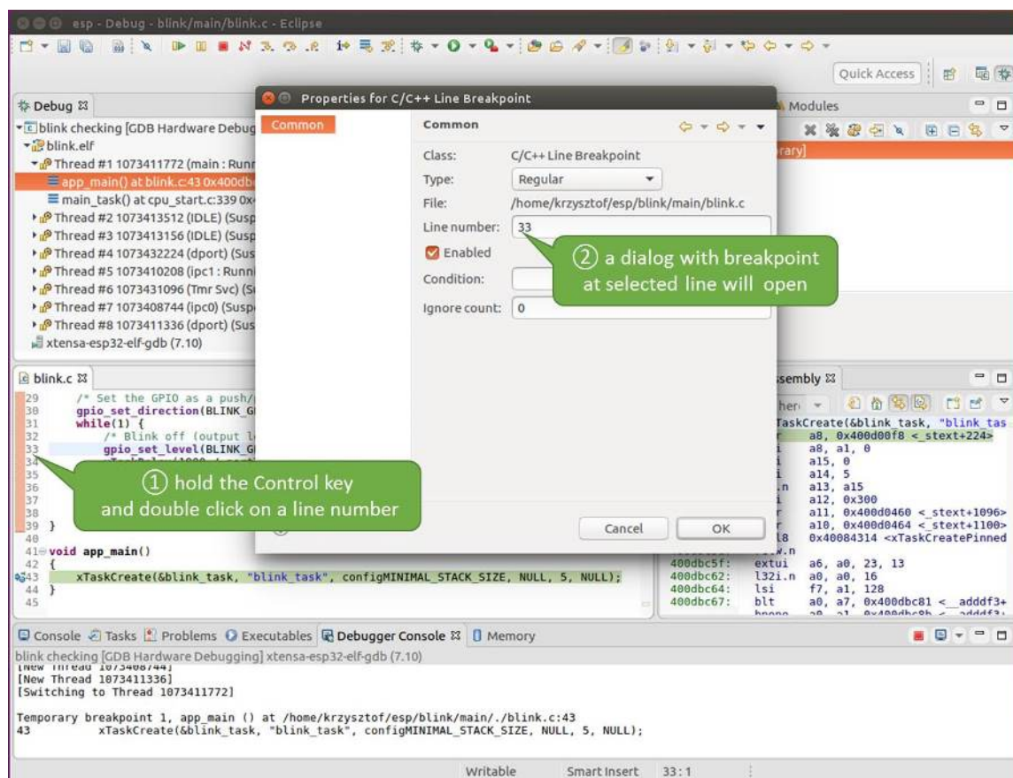
Fig. 19: Setting a breakpoint
