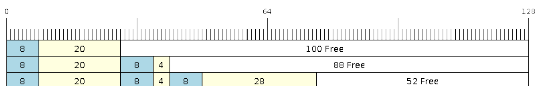
Fig. 30: Sending items to No-Split or Allow-Split ring buffers
