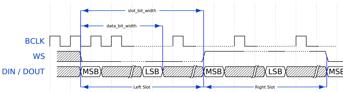
Standard MSB Timing Diagram
