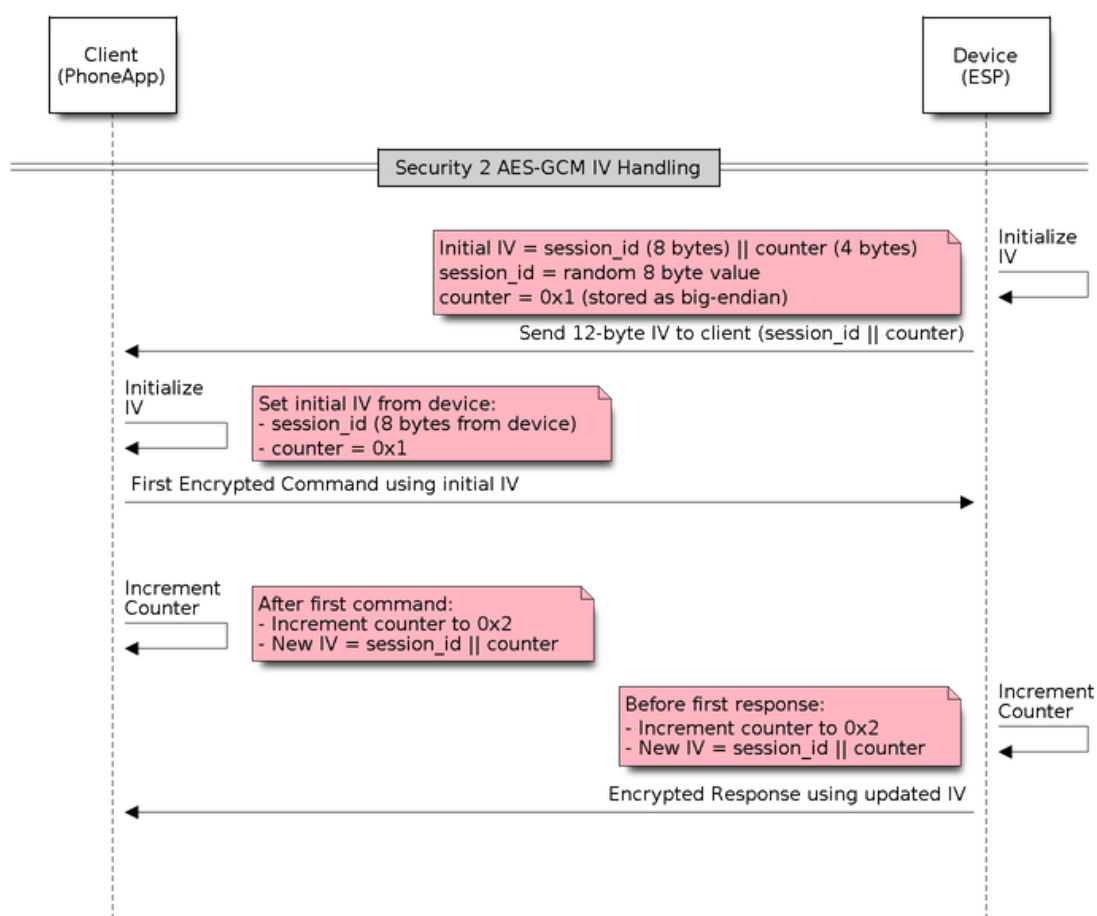
Fig. 30: Security 2 AES-GCM IV Handling
