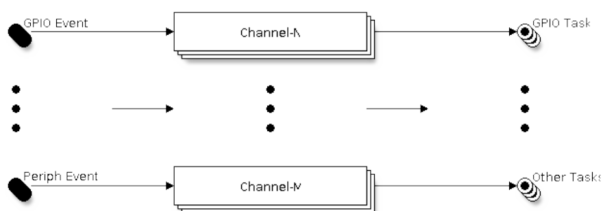
Fig. 5: ETM channels Overview
