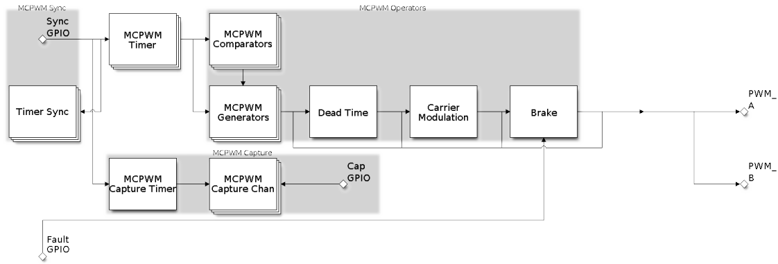
Fig. 9: MCPWM Overview
