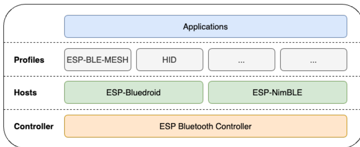
Fig. 2: ESP32-H2 Bluetooth LE Stack Architecture
