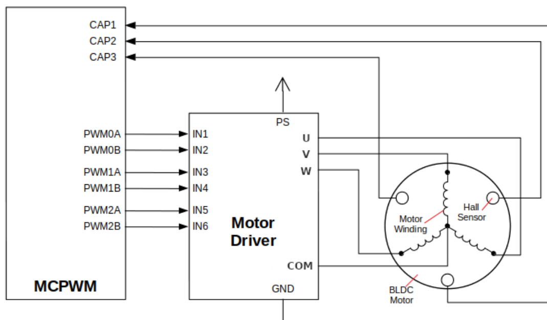
Fig. 11: MCPWM BLDC with Hall Sensor
