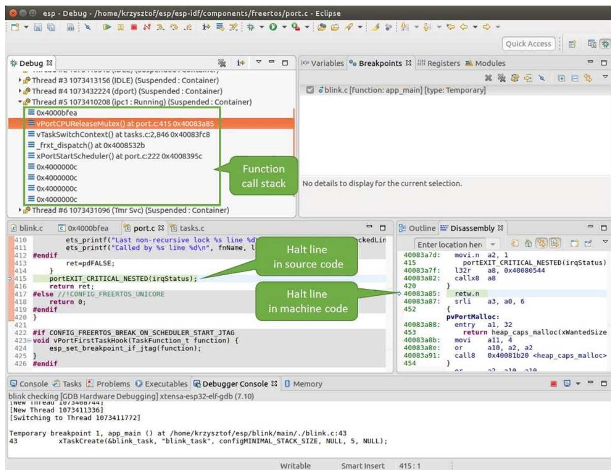
Fig. 48: Navigate through the call stack
