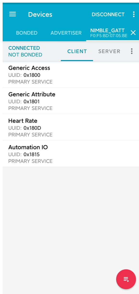
Fig. 8: GATT Services List
