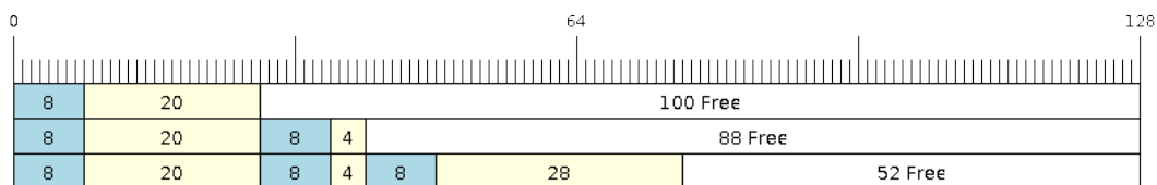
Fig. 24: Sending items to No-Split or Allow-Split ring buffers
