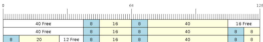
Fig. 28: Wrap around in Allow-Split buffers
