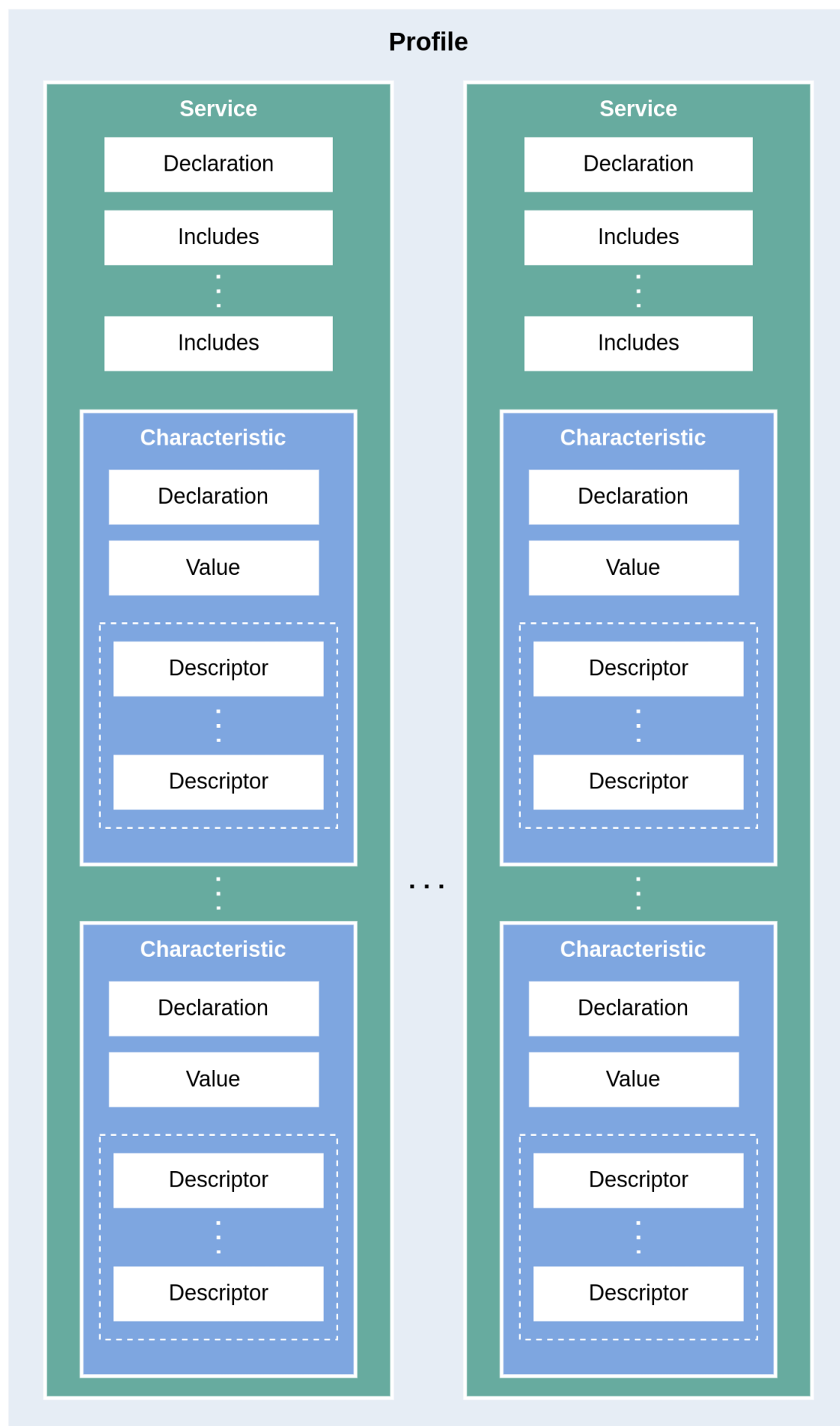
Fig. 5: GATT Hierarchical Architecture
