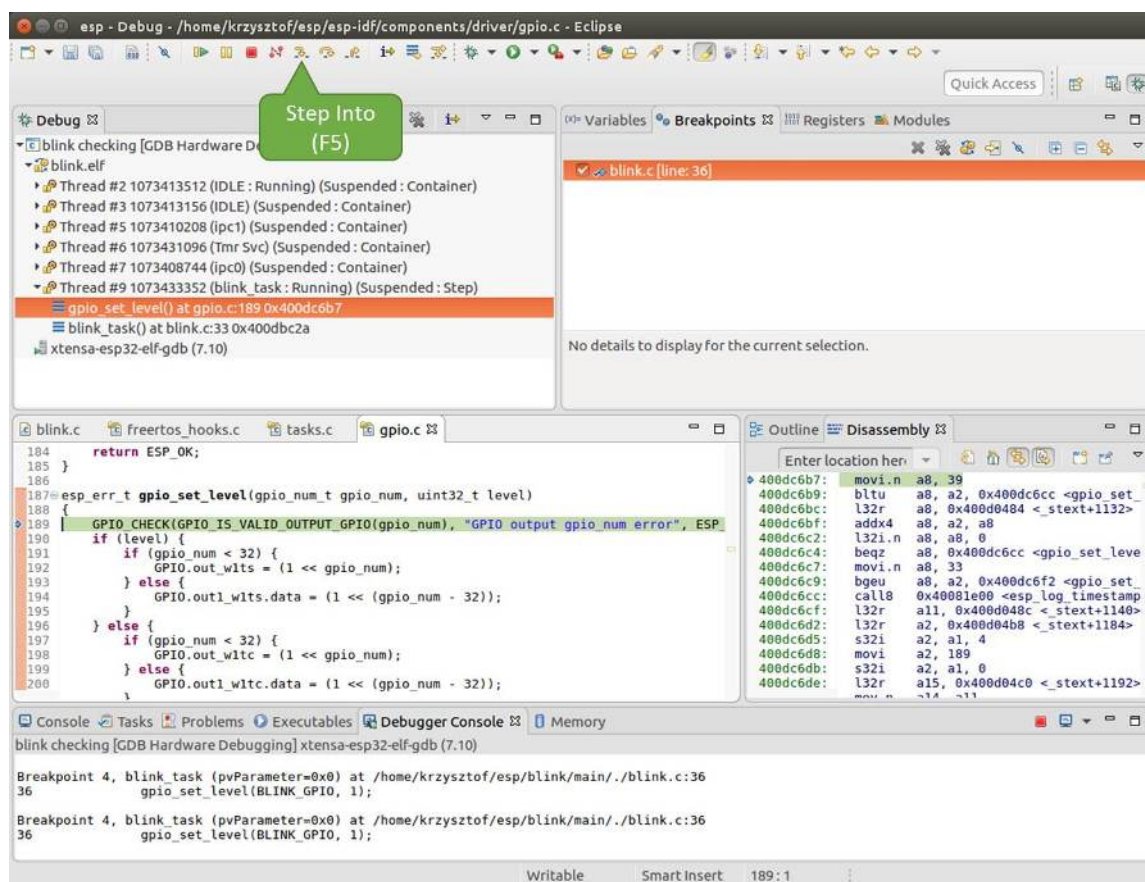
Fig. 53: Stepping through the code with "Step Into (F5)"
