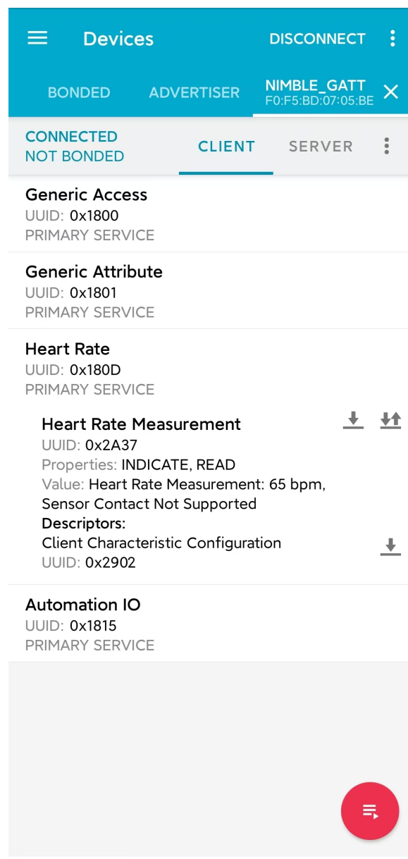
Fig. 12: Read Heart Rate Characteristic Data
