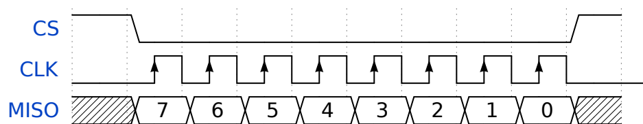
SPI normal mode 0
