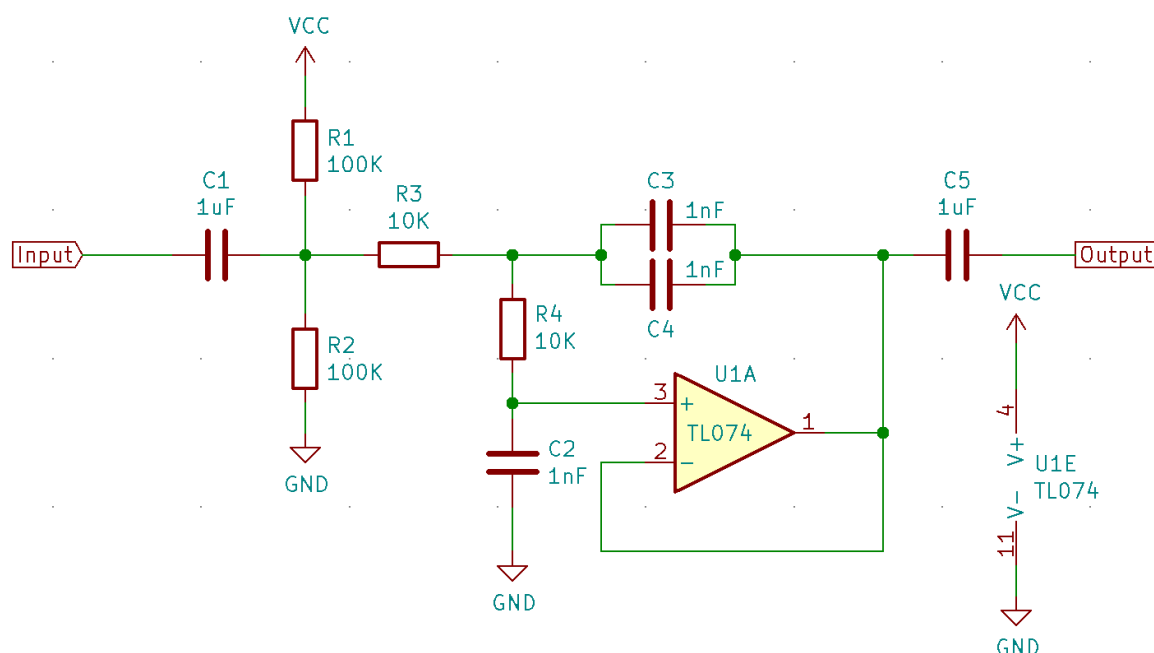
Fig. 18: Sallen-Key Low Pass Filter
