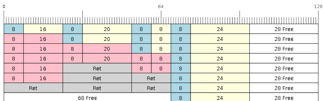
Fig. 30: Retrieving/Returning items in No-Split and Allow-Split ring buffers
