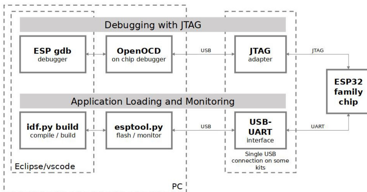
Fig. 41: JTAG debugging - overview diagram
