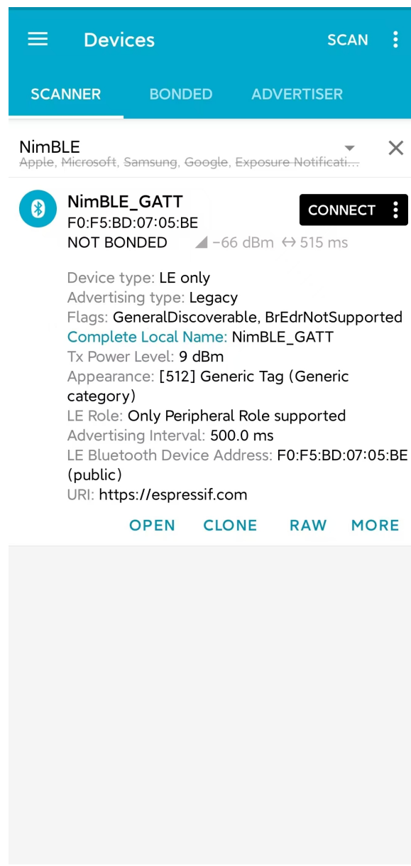
Fig. 7: Advertising Data Details
