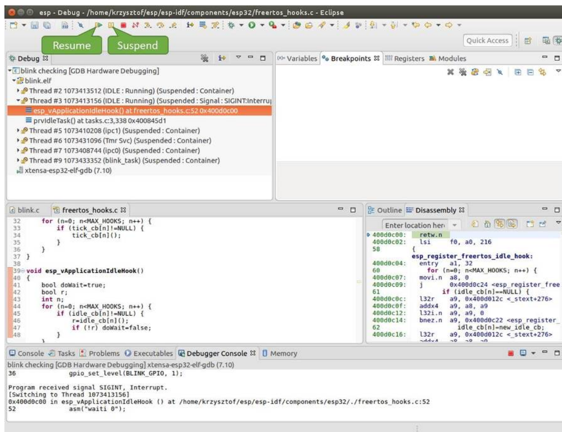
Fig. 51: Target halted manually
