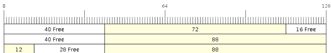
Fig. 29: Wrap around in byte buffers
