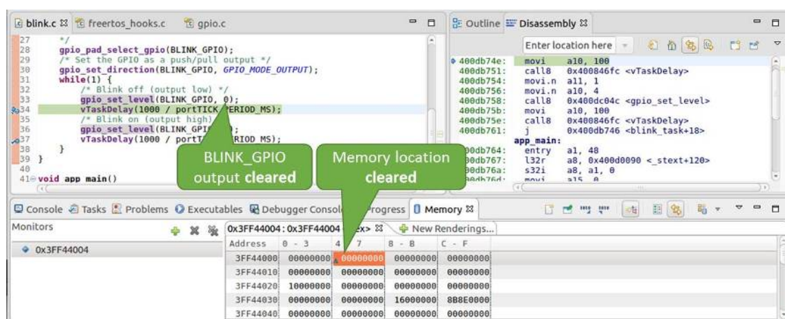
Fig. 55: Observing memory location 0x3FF44004 changing one bit to "OFF"
