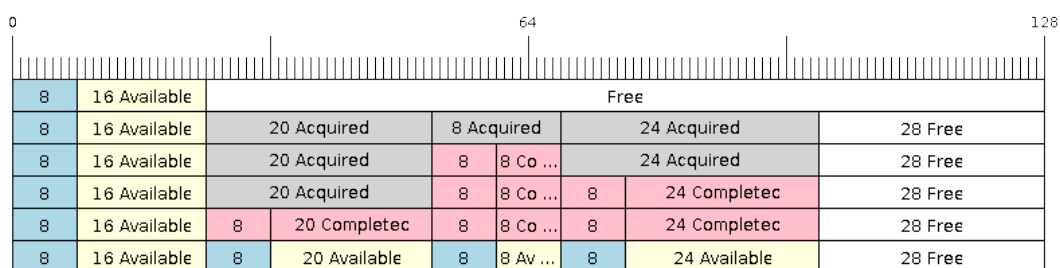
Fig. 26: SendAcquire / SendComplete items in No-Split ring buffers
