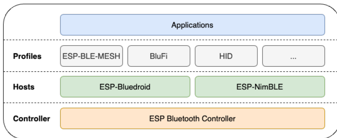
Fig. 2: ESP32-C3 Bluetooth LE Stack Architecture
