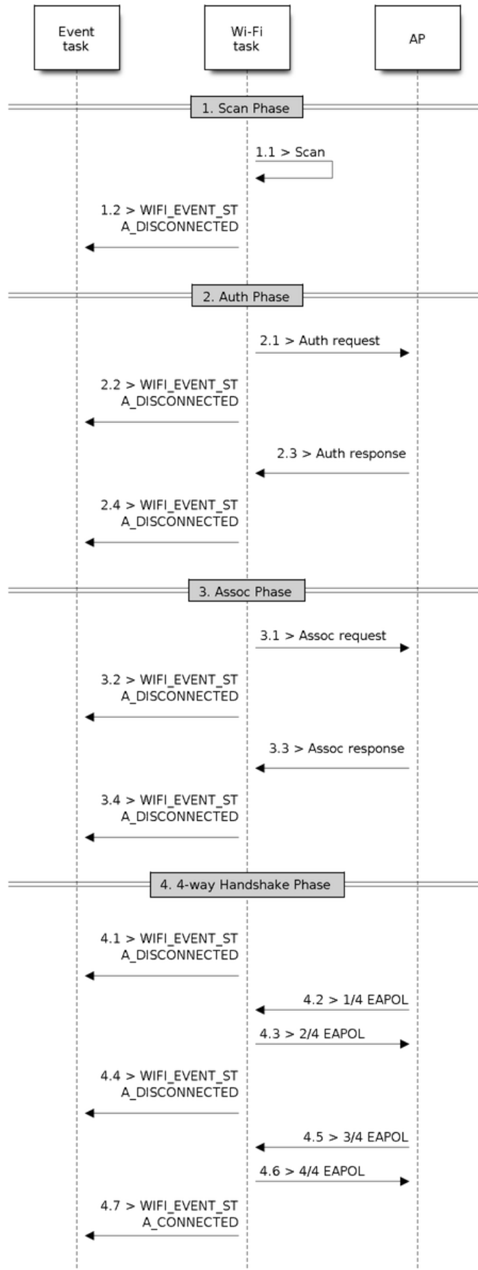
Fig. 86: Wi-Fi Station Connecting Process
