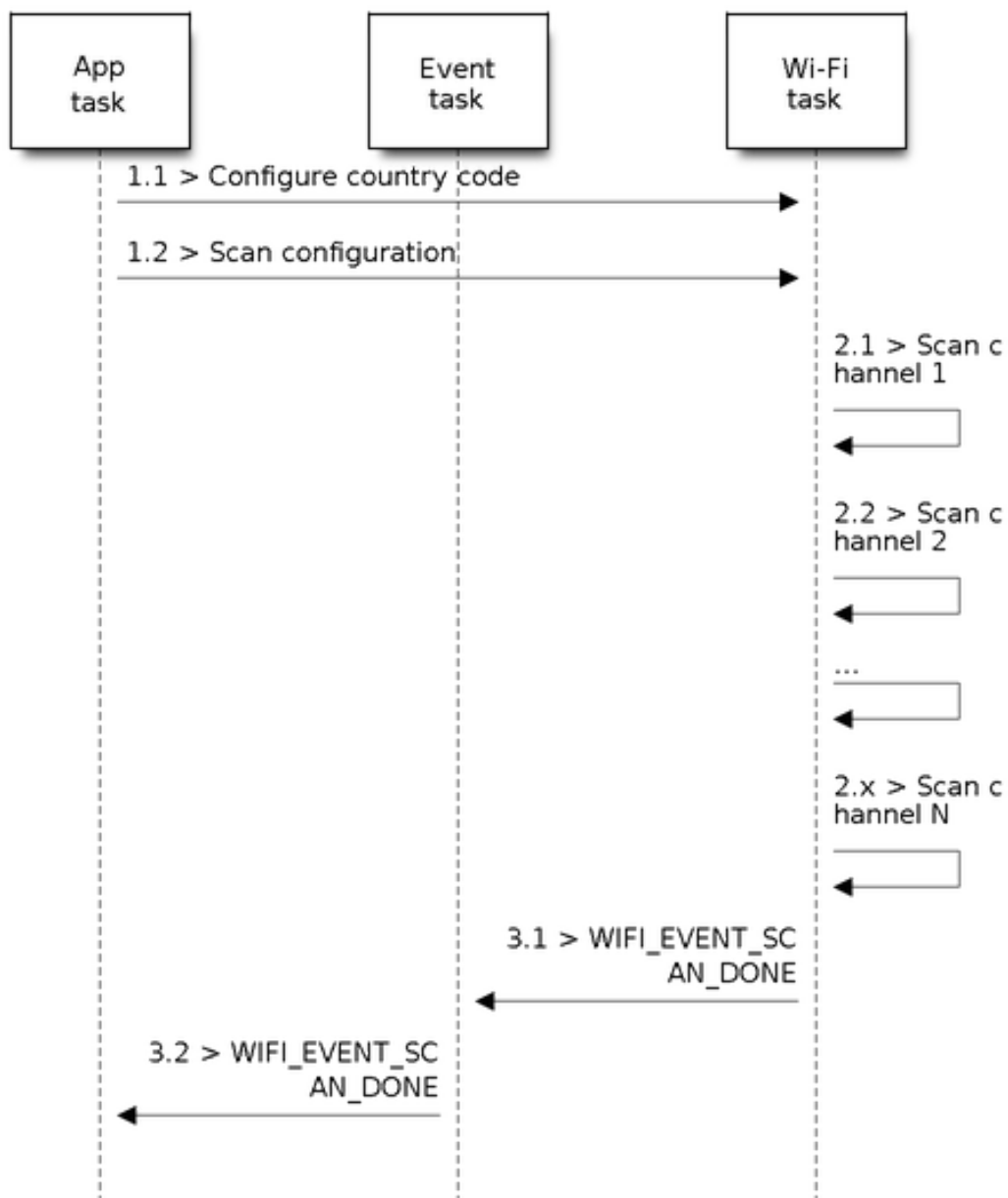
Fig. 83: Foreground Scan of all Wi-Fi Channels
