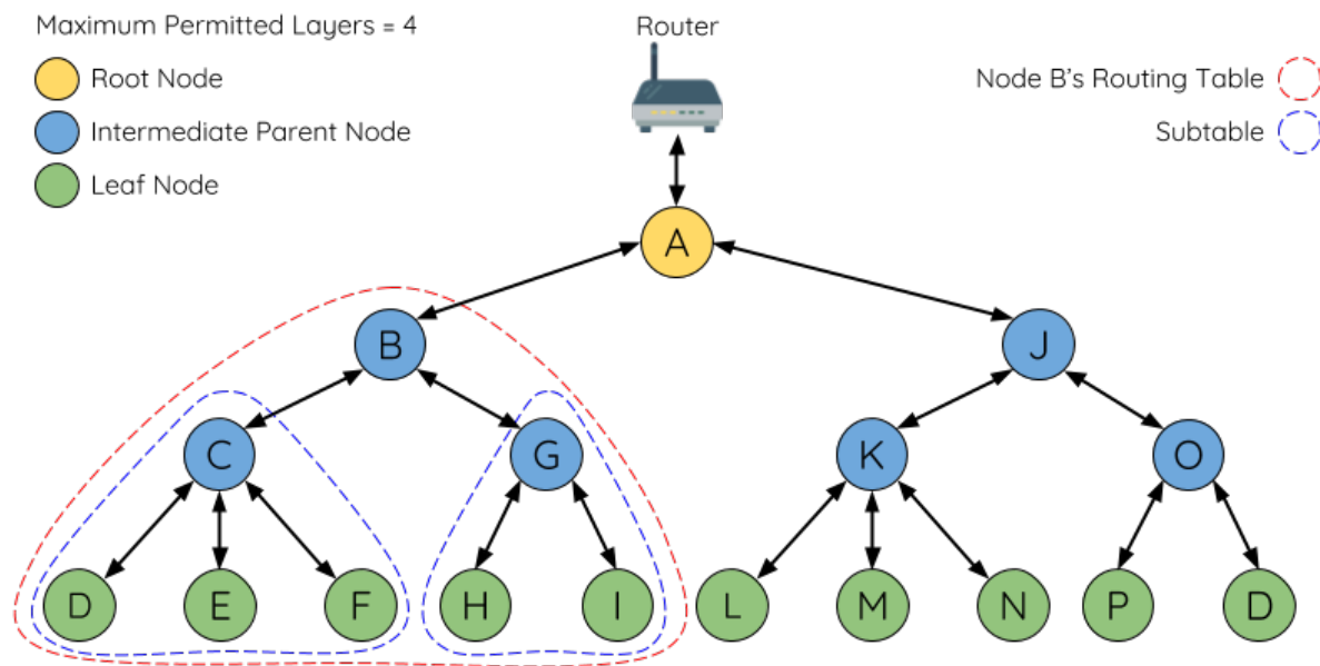
Fig. 51: ESP-WIFI-MESH Routing Tables Example
