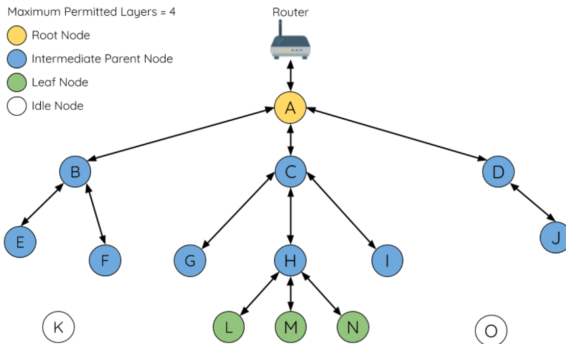
Fig. 48: ESP-WIFI-MESH Node Types
