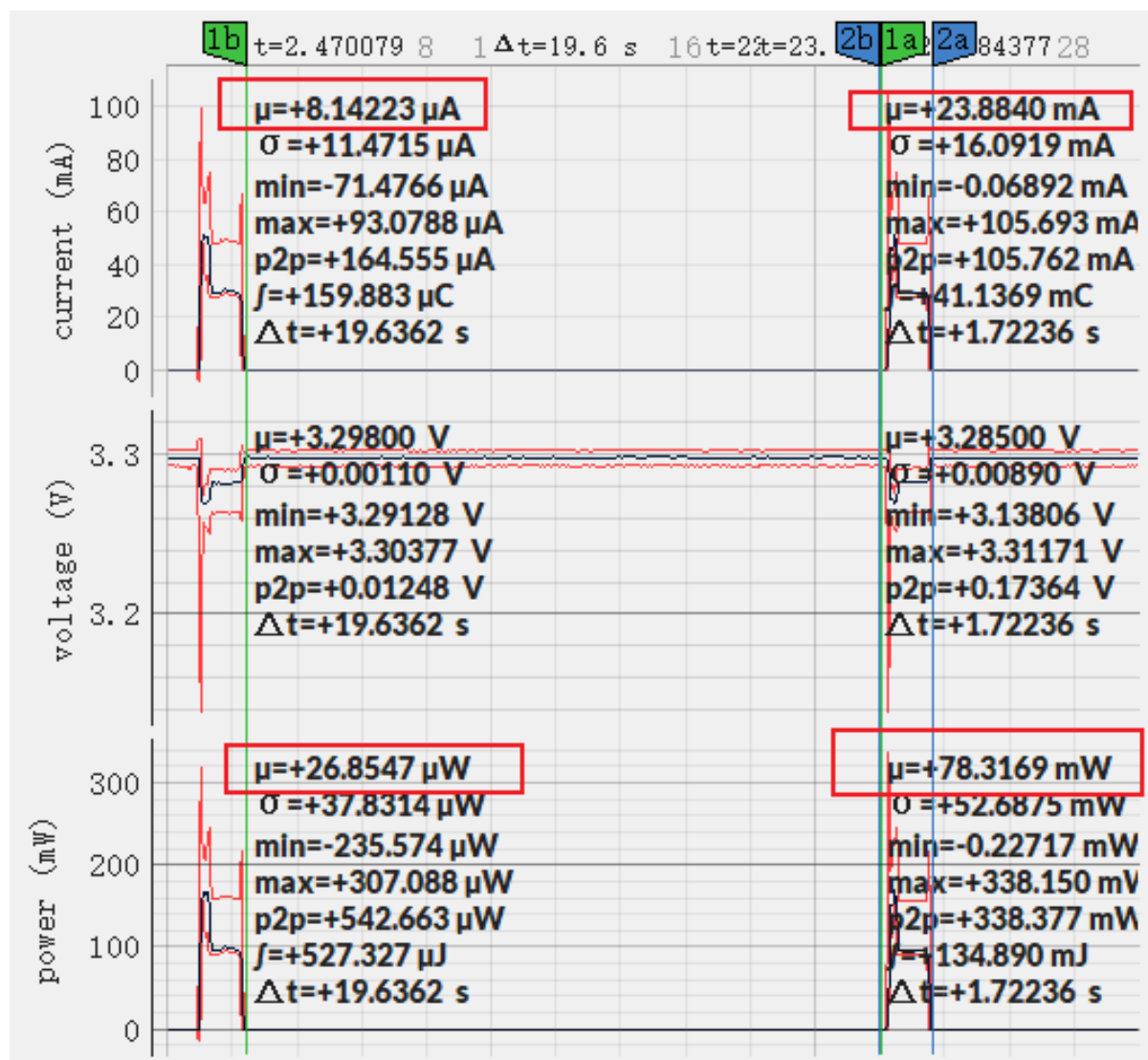
Fig. 43: Current Waveform of ESP32-S3-WROOM-1 (click to enlarge)
