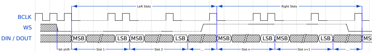
TDM Philips Timing Diagram
