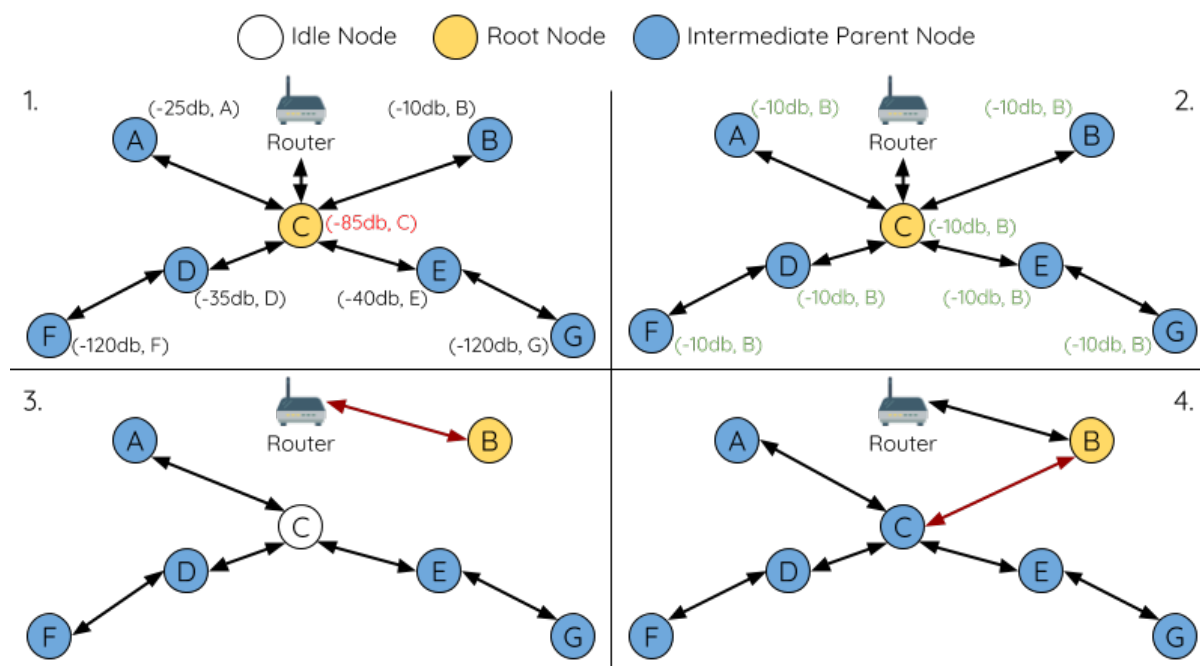
Fig. 58: Root Node Switch Example
