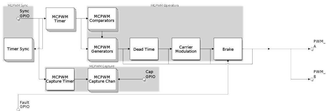
Fig. 17: MCPWM Overview
