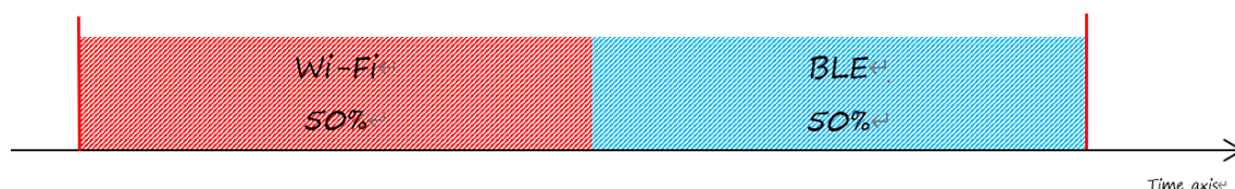
Fig. 39: Time Slice Under the Status of Wi-Fi CONNECTED and BLE CONNECTED
