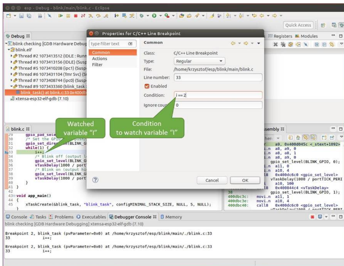
Fig. 80: Setting a conditional breakpoint
