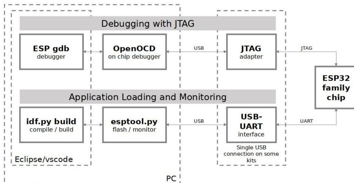
Fig. 63: JTAG debugging - overview diagram
