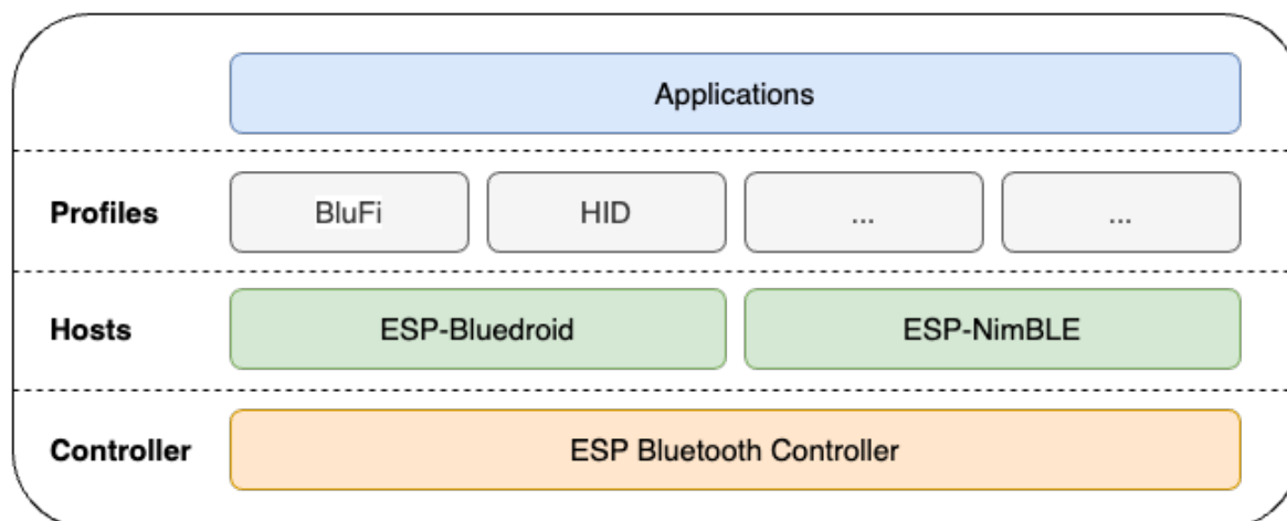
Fig. 2: ESP32-C2 Bluetooth LE Stack Architecture
