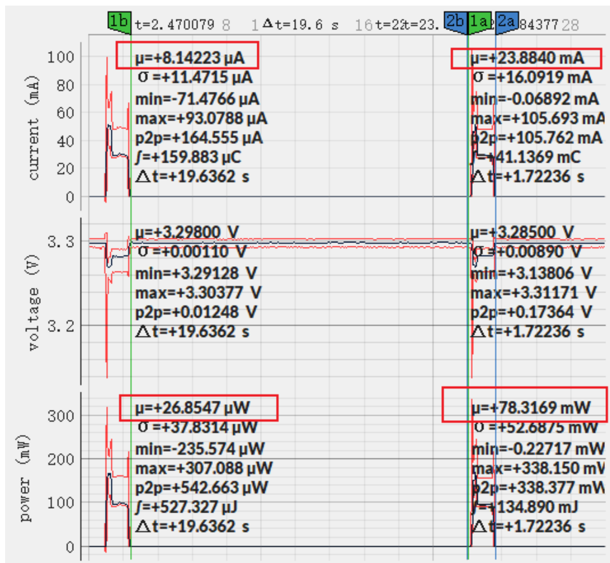
Fig. 31: Current Waveform of ESP32-S3-WROOM-1 (click to enlarge)
