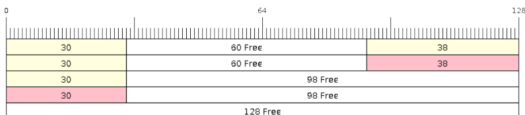
Fig. 21: Retrieving/Returning data in byte buffers
