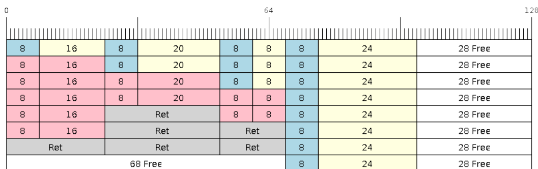
Fig. 20: Retrieving/Returning items in No-Split and Allow-Split ring buffers
