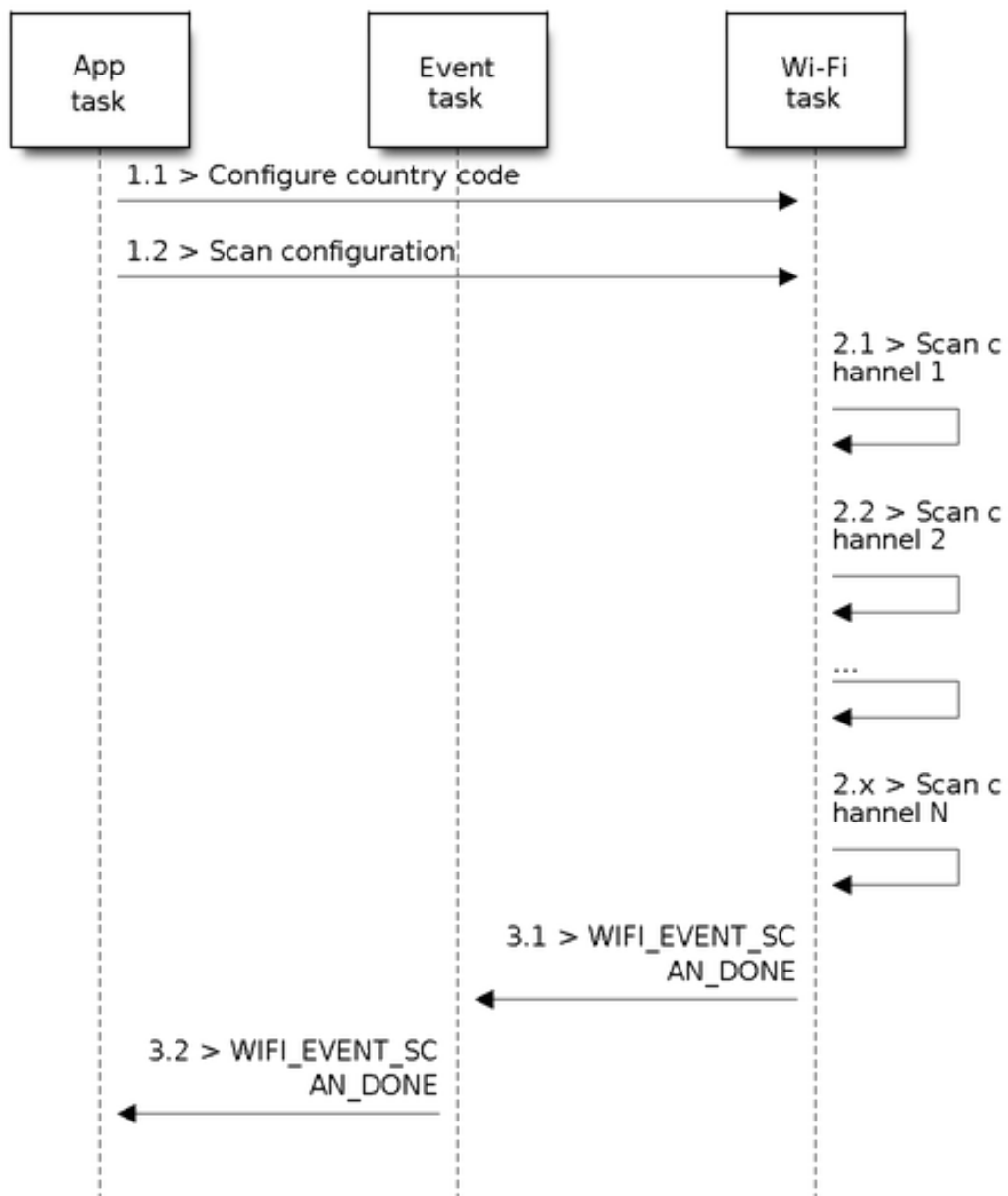
Fig. 55: Foreground Scan of all Wi-Fi Channels
