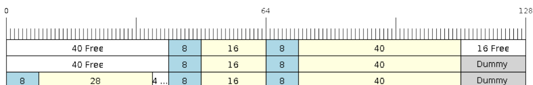
Fig. 18: Wrap around in No-Split buffers
