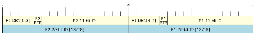
Fig. 30: Bit layout of dual filter mode (Right side MSBit)
