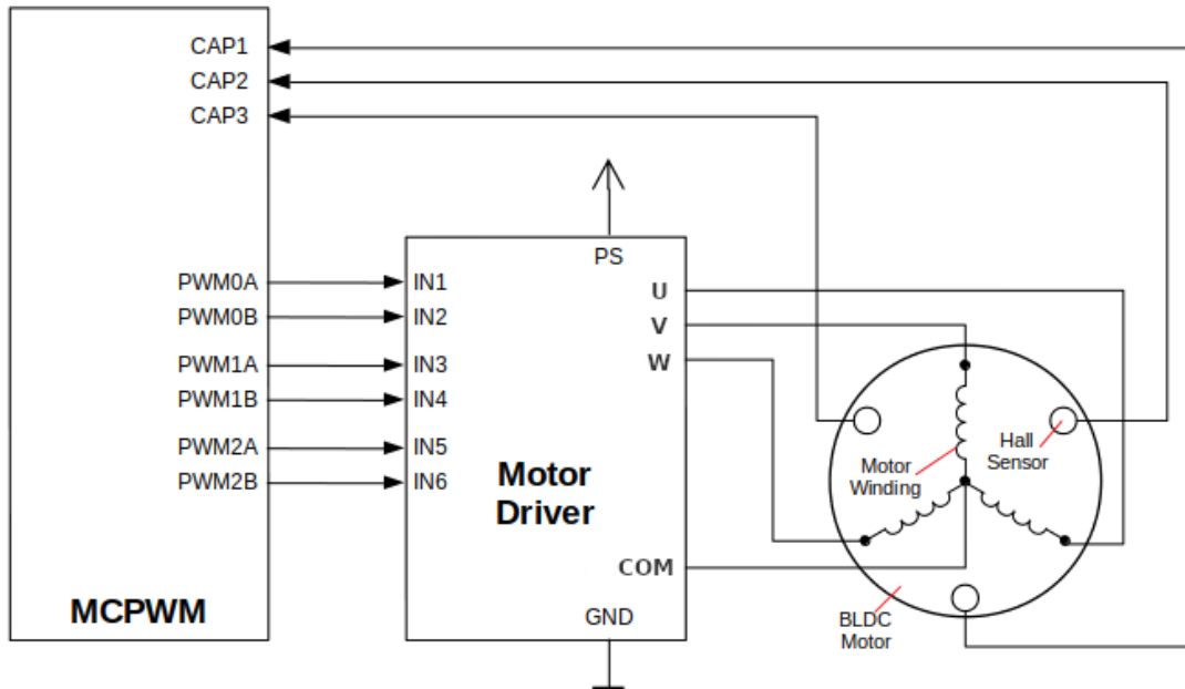
Fig. 19: MCPWM BLDC with Hall Sensor
