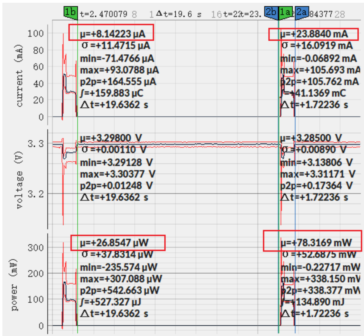
Fig. 22: Current Waveform of ESP32-S3-WROOM-1 (click to enlarge)
