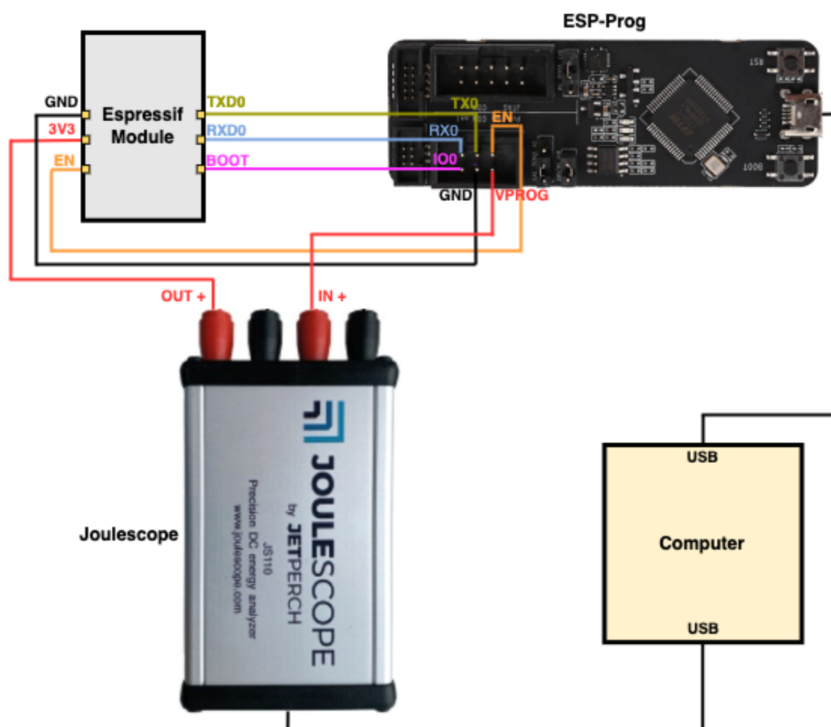
Fig. 21: Hardware Connection (click to enlarge)
