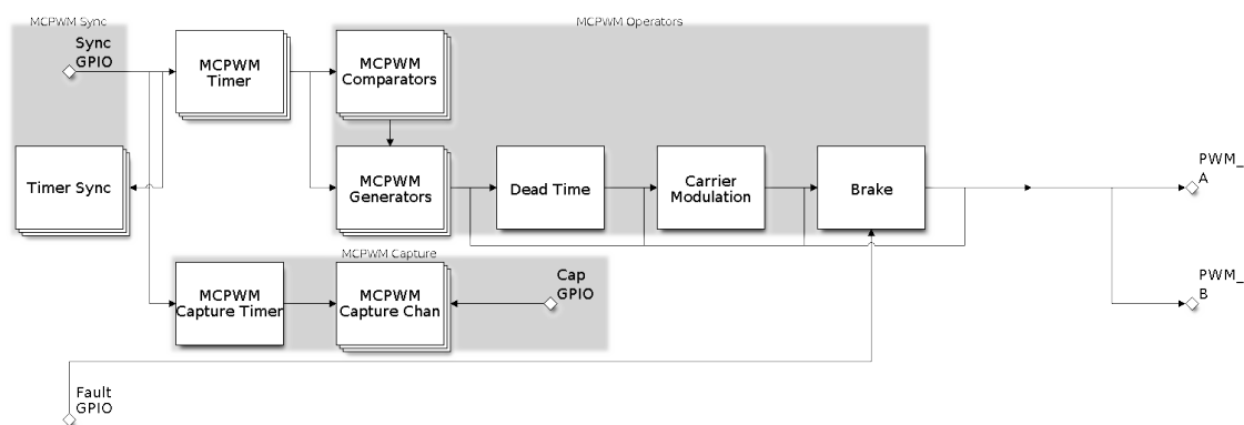
Fig. 15: MCPWM Overview
