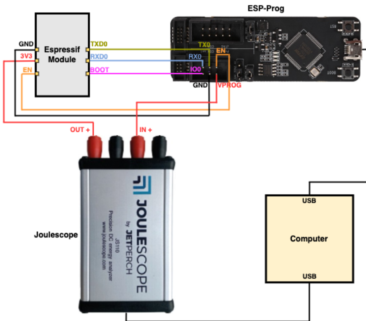
Fig. 41: Hardware Connection (click to enlarge)
