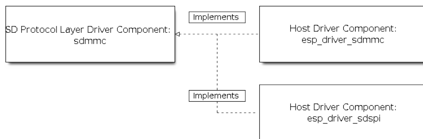
Fig. 30: SD Host Side Component Architecture
