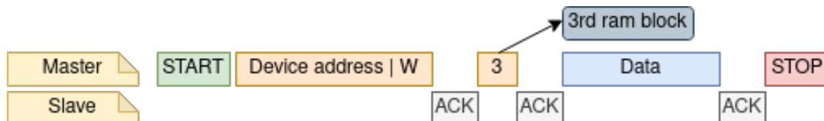
Fig. 11: Put data in I2C slave RAM
