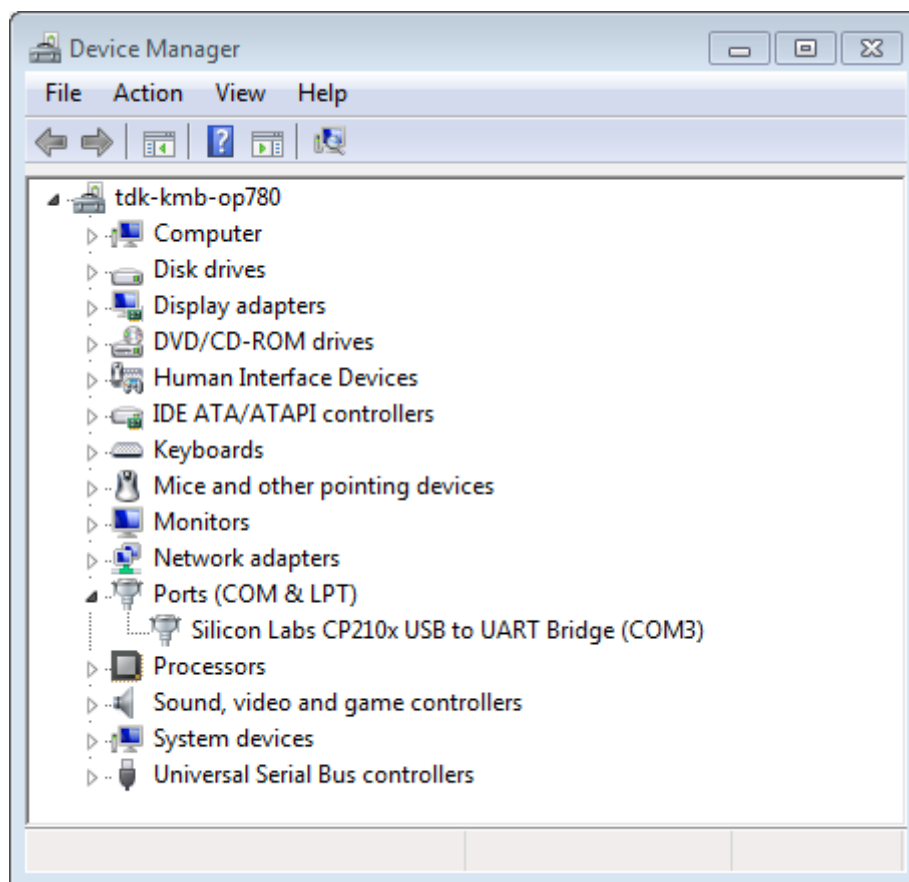
Fig. 32: USB to UART bridge of ESP32-DevKitC in Windows Device Manager
