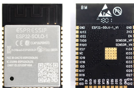
Fig. 4: ESP32-SOLO-1 module (front and back)
