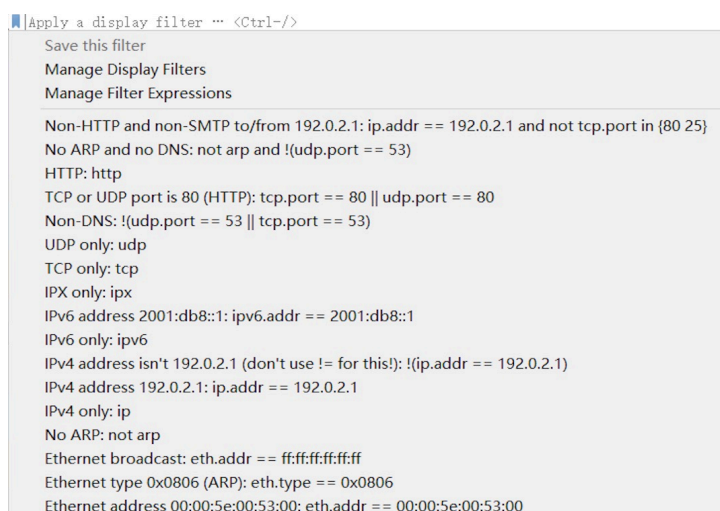
Fig. 47: Display Filter Dialogue Box
