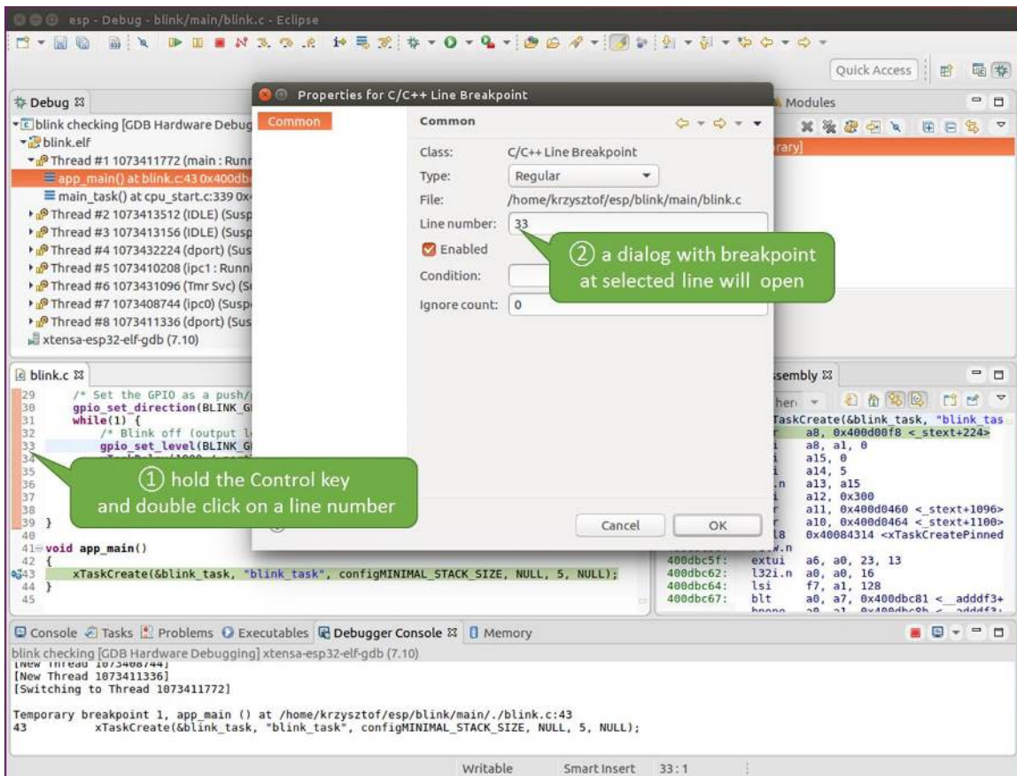
Fig. 26: Setting a breakpoint
