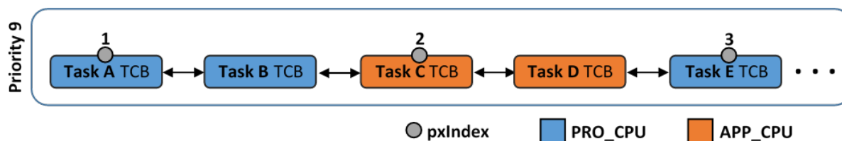
Fig. 16: Illustration of pxIndex behavior in ESP-IDF FreeRTOS
