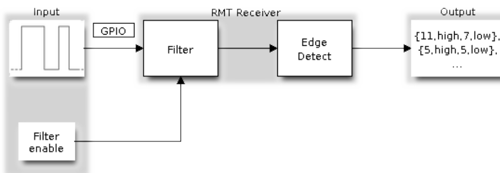
Fig. 16: RMT Receiver Overview
