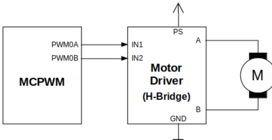
Fig. 13: Example of Brushed DC Motor Control with MCPWM
