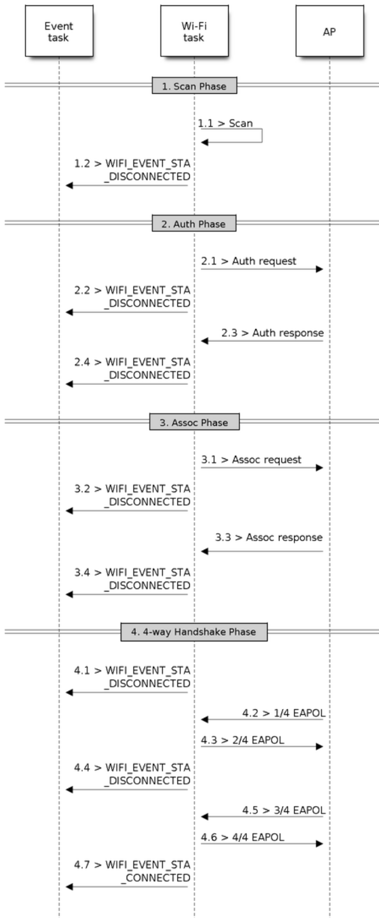
Fig. 59: Wi-Fi Station Connecting Process
