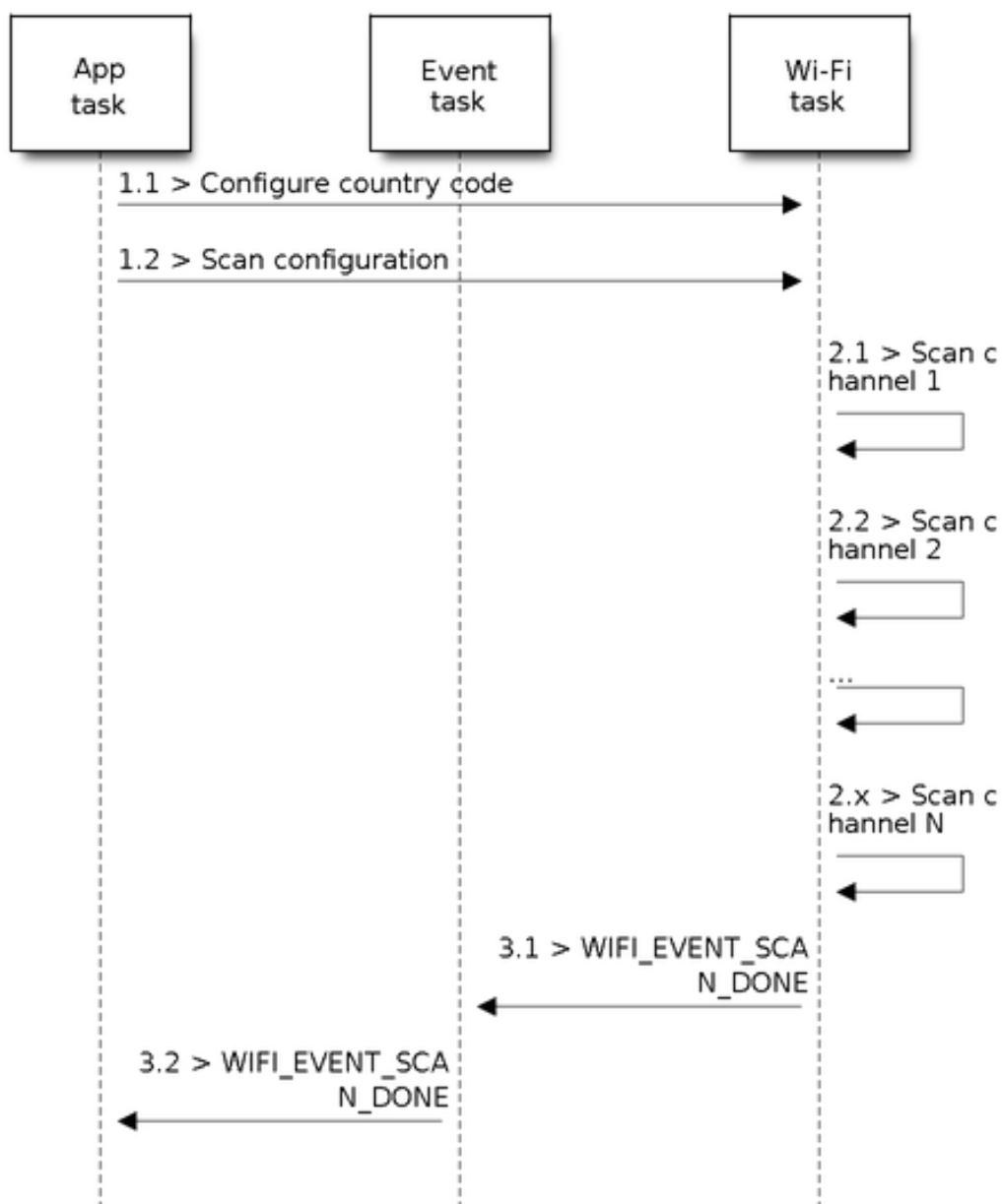
Fig. 56: Foreground Scan of all Wi-Fi Channels
