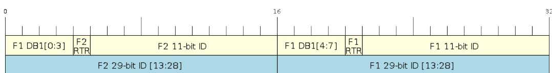
Fig. 16: Bit layout of dual filter mode (Right side MSBit)
