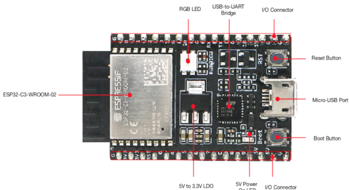
Fig. 7: ESP32-C3-DevKitC-02 - front
