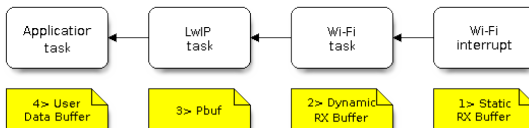
Fig. 62: RX Buffer Allocation
