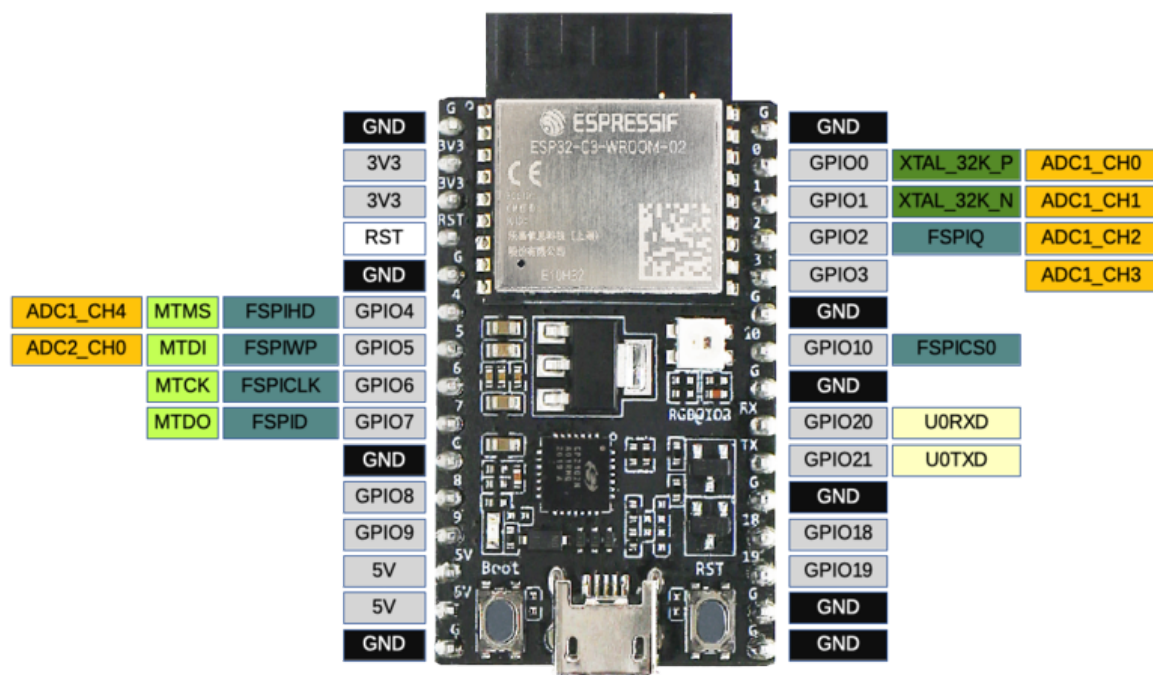
Fig. 9: ESP32-C3-DevKitC-02 Pin Layout
