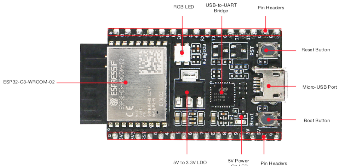
Fig. 7: ESP32-C3-DevKitC-02 - front
