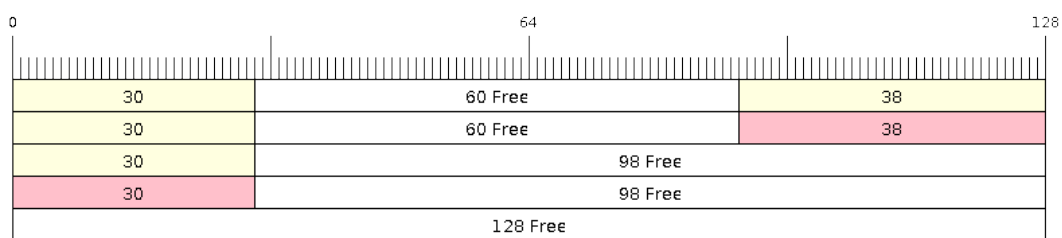
Fig. 29: Retrieving/Returning data in byte buffers
