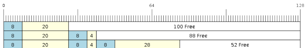
Fig. 22: Sending items to No-Split or Allow-Split ring buffers
