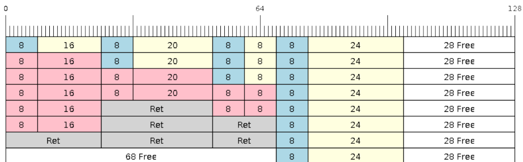
Fig. 28: Retrieving/Returning items in No-Split and Allow-Split ring buffers
