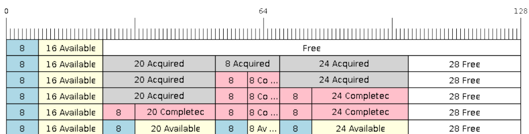
Fig. 29: SendAcquire / SendComplete items in No-Split ring buffers
