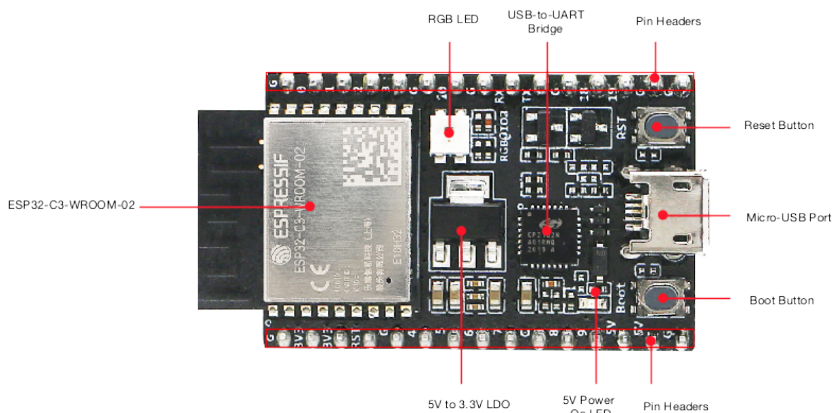
Fig. 7: ESP32-C3-DevKitC-02 - front
